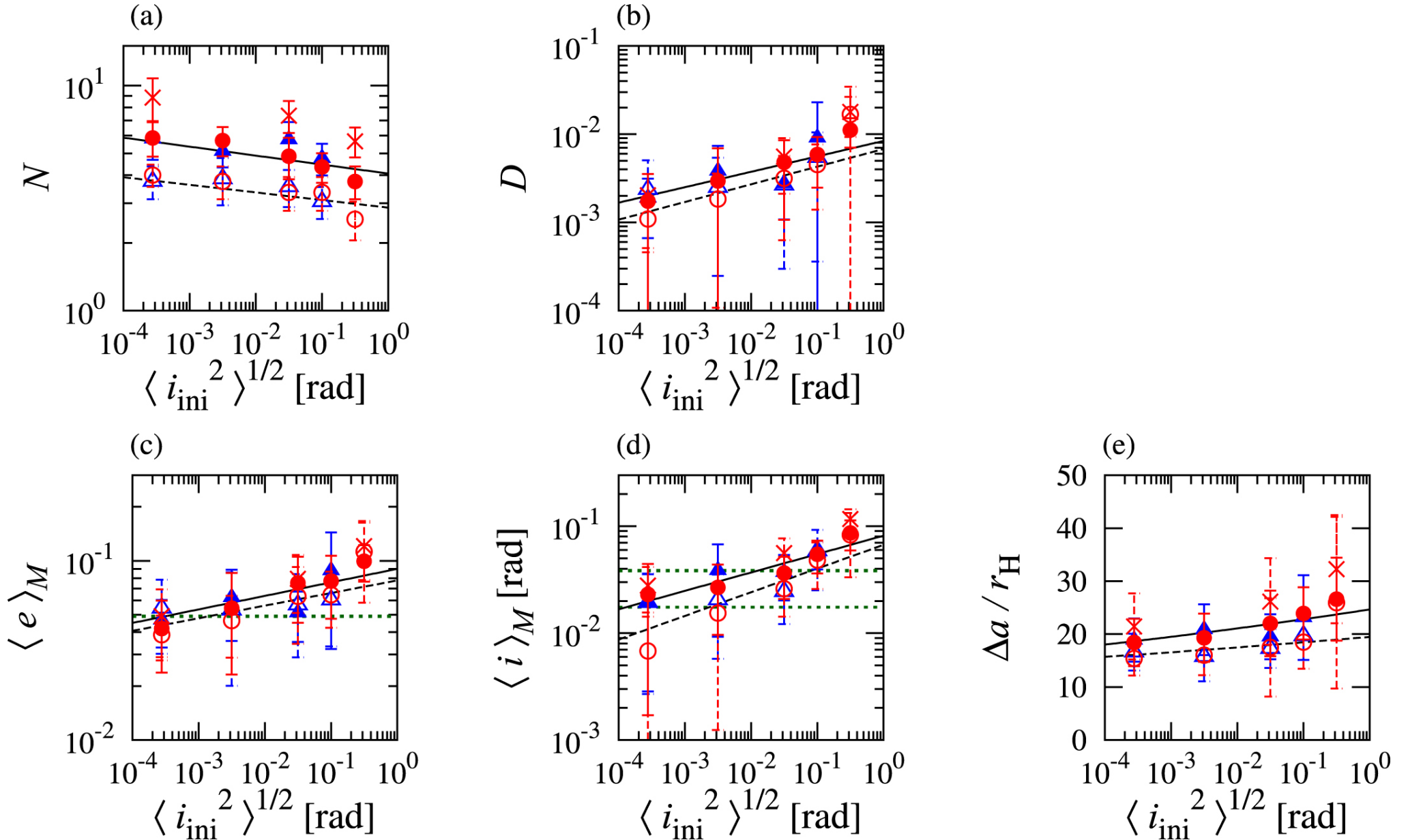
Figure 9. from Formation of Close-in Super-Earths by Giant Impacts: Effects of Initial Eccentricities and Inclinations of Protoplanets null 2017 AJ 154 27 doi:10.3847/1538-3881/aa74c7 https://dx.doi.org/10.3847/1538-3881/aa74c7 © 2017. The American Astronomical Society. All rights reserved.
