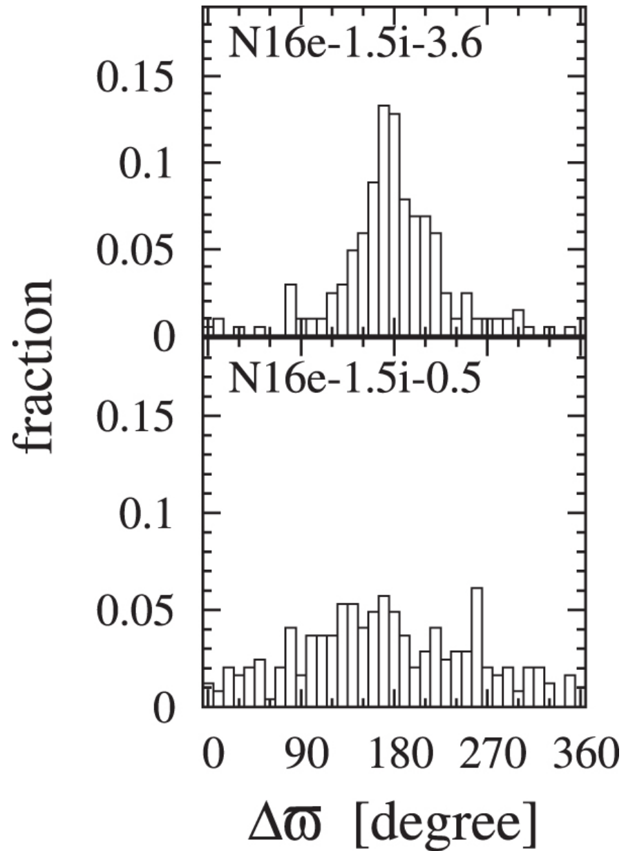
Figure 8. from Formation of Close-in Super-Earths by Giant Impacts: Effects of Initial Eccentricities and Inclinations of Protoplanets null 2017 AJ 154 27 doi:10.3847/1538-3881/aa74c7 https://dx.doi.org/10.3847/1538-3881/aa74c7 © 2017. The American Astronomical Society. All rights reserved.
