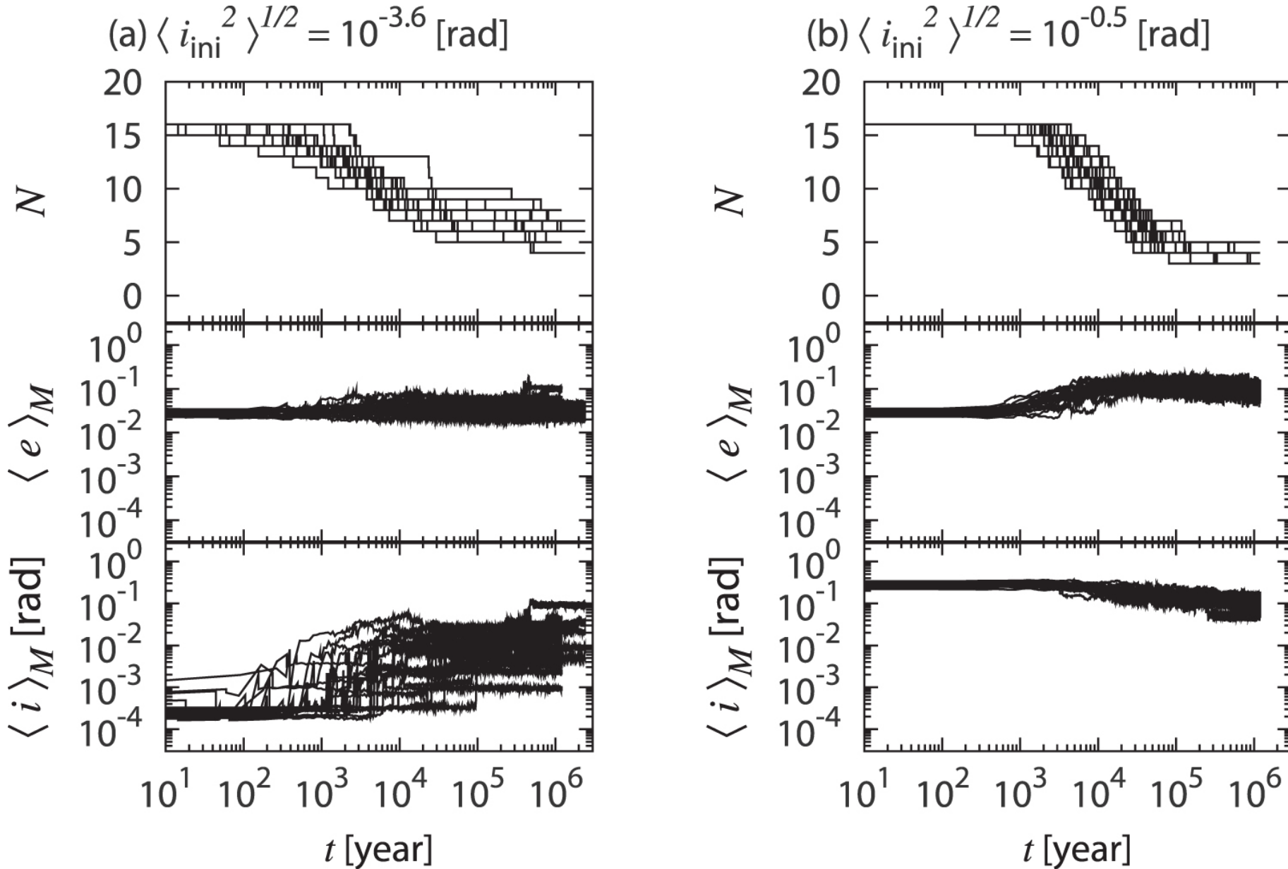
Figure 6. from Formation of Close-in Super-Earths by Giant Impacts: Effects of Initial Eccentricities and Inclinations of Protoplanets null 2017 AJ 154 27 doi:10.3847/1538-3881/aa74c7 https://dx.doi.org/10.3847/1538-3881/aa74c7 © 2017. The American Astronomical Society. All rights reserved.
