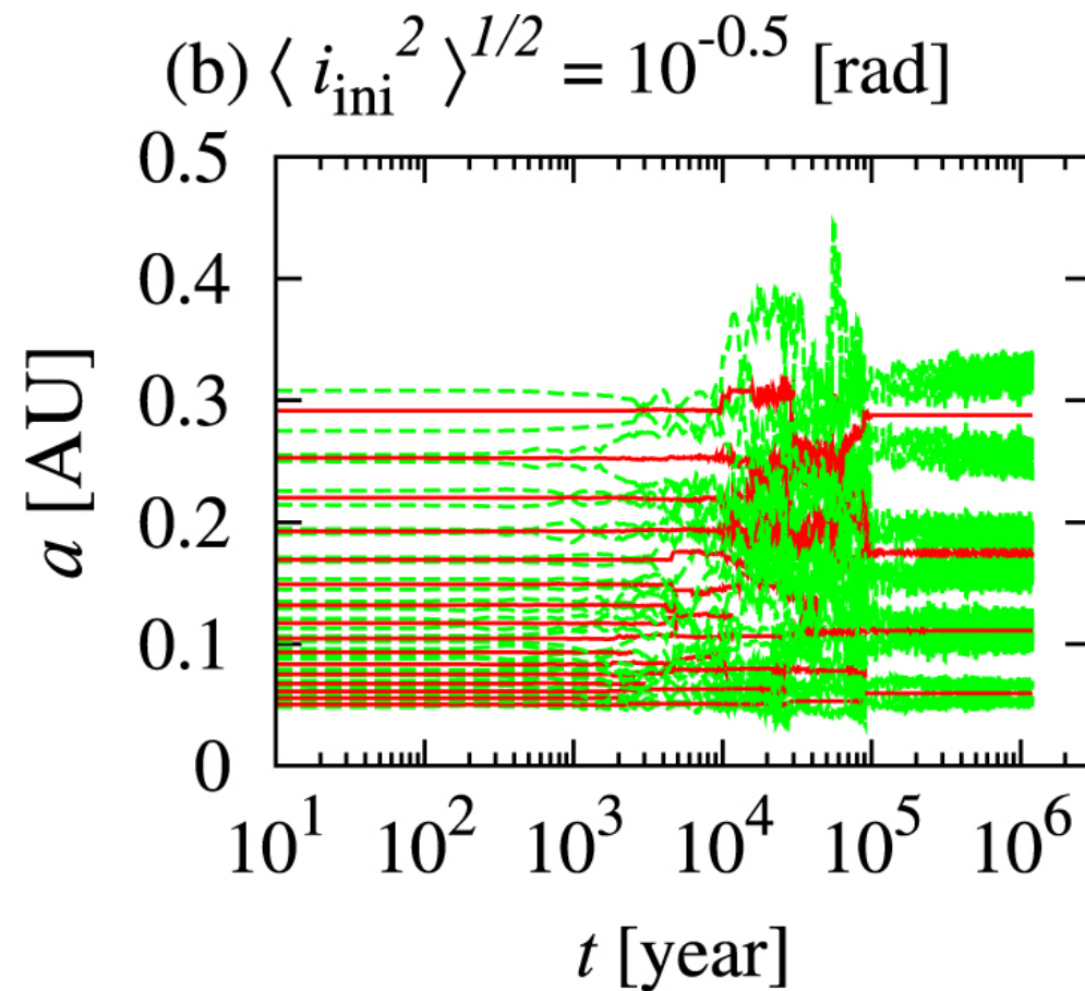
Figure 5. from Formation of Close-in Super-Earths by Giant Impacts: Effects of Initial Eccentricities and Inclinations of Protoplanets null 2017 AJ 154 27 doi:10.3847/1538-3881/aa74c7 https://dx.doi.org/10.3847/1538-3881/aa74c7 © 2017. The American Astronomical Society. All rights reserved.
