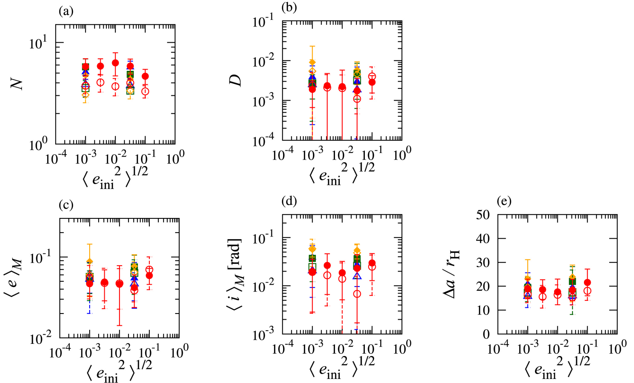
Figure 4. from Formation of Close-in Super-Earths by Giant Impacts: Effects of Initial Eccentricities and Inclinations of Protoplanets null 2017 AJ 154 27 doi:10.3847/1538-3881/aa74c7 https://dx.doi.org/10.3847/1538-3881/aa74c7 © 2017. The American Astronomical Society. All rights reserved.
