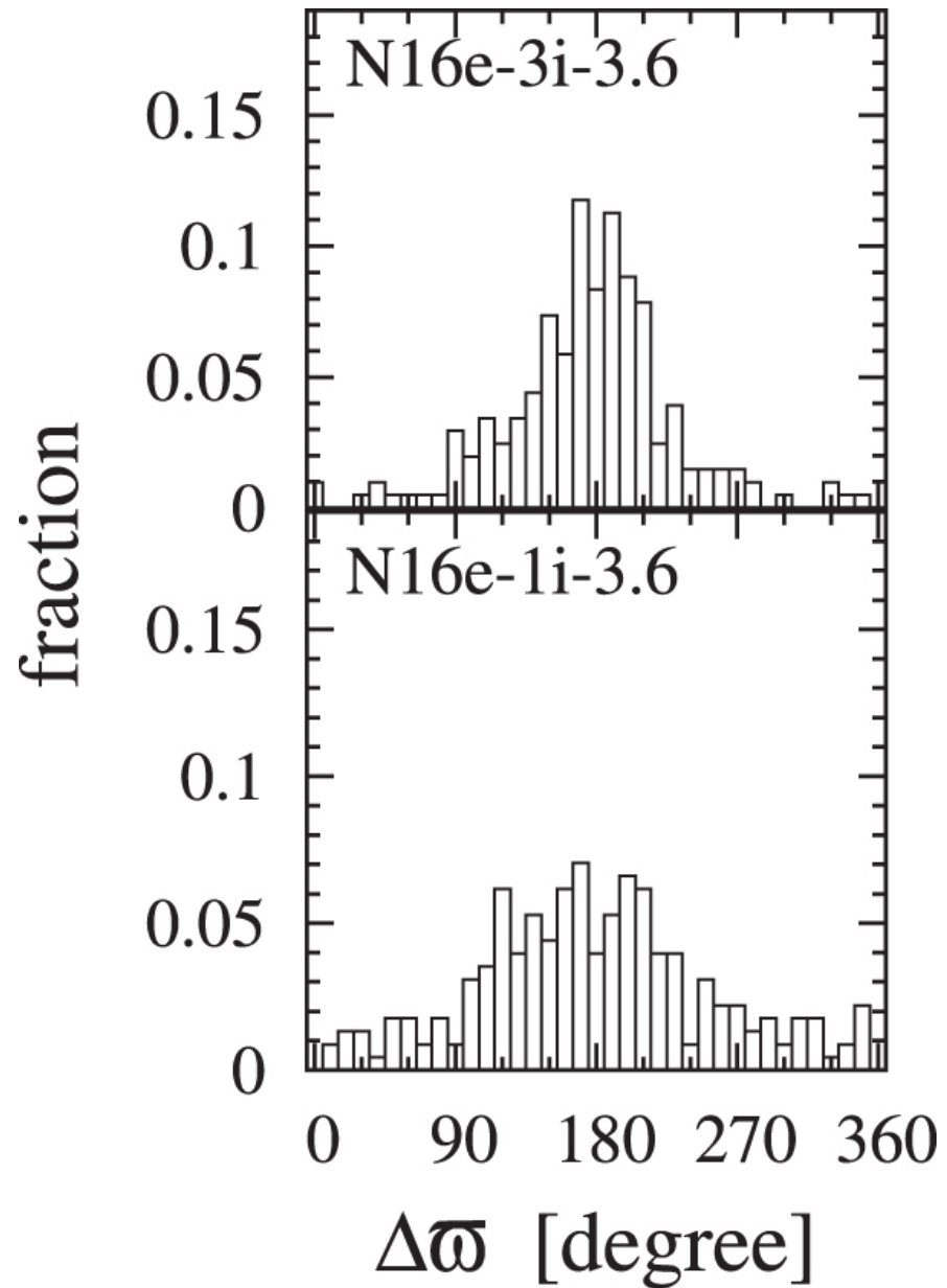
Figure 3. from Formation of Close-in Super-Earths by Giant Impacts: Effects of Initial Eccentricities and Inclinations of Protoplanets null 2017 AJ 154 27 doi:10.3847/1538-3881/aa74c7 https://dx.doi.org/10.3847/1538-3881/aa74c7 © 2017. The American Astronomical Society. All rights reserved.
