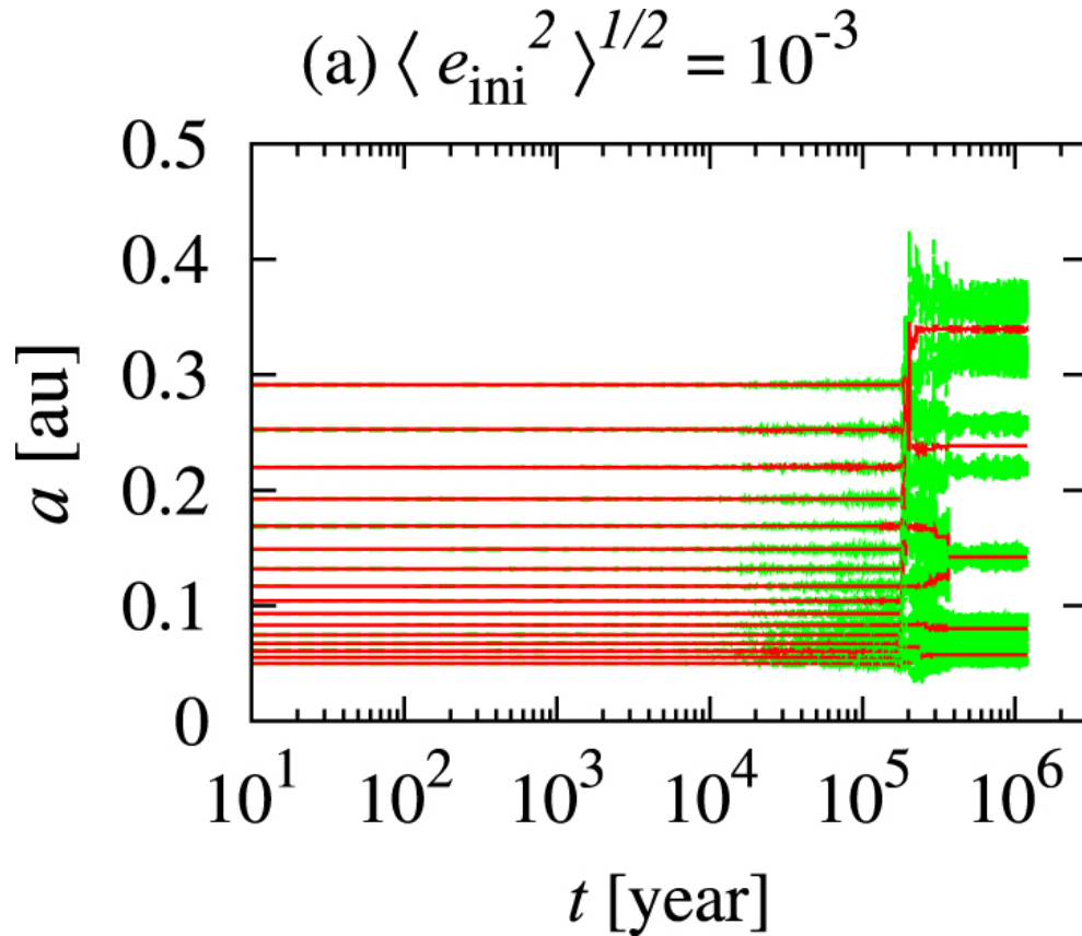
Figure 1. from Formation of Close-in Super-Earths by Giant Impacts: Effects of Initial Eccentricities and Inclinations of Protoplanets null 2017 AJ 154 27 doi:10.3847/1538-3881/aa74c7 https://dx.doi.org/10.3847/1538-3881/aa74c7 © 2017. The American Astronomical Society. All rights reserved.
