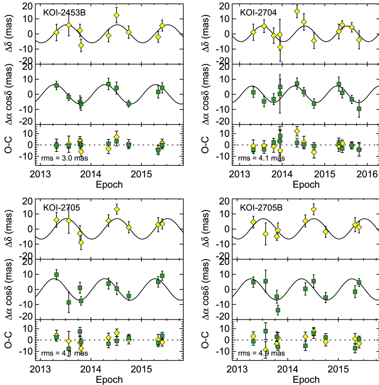
Figure 9. from The Gold Standard: Accurate Stellar and Planetary Parameters for Eight Kepler M Dwarf Systems Enabled by Parallaxes null 2017 AJ 153 267 doi:10.3847/1538-3881/aa7140 https://dx.doi.org/10.3847/1538-3881/aa7140 © 2017. The American Astronomical Society. All rights reserved.
