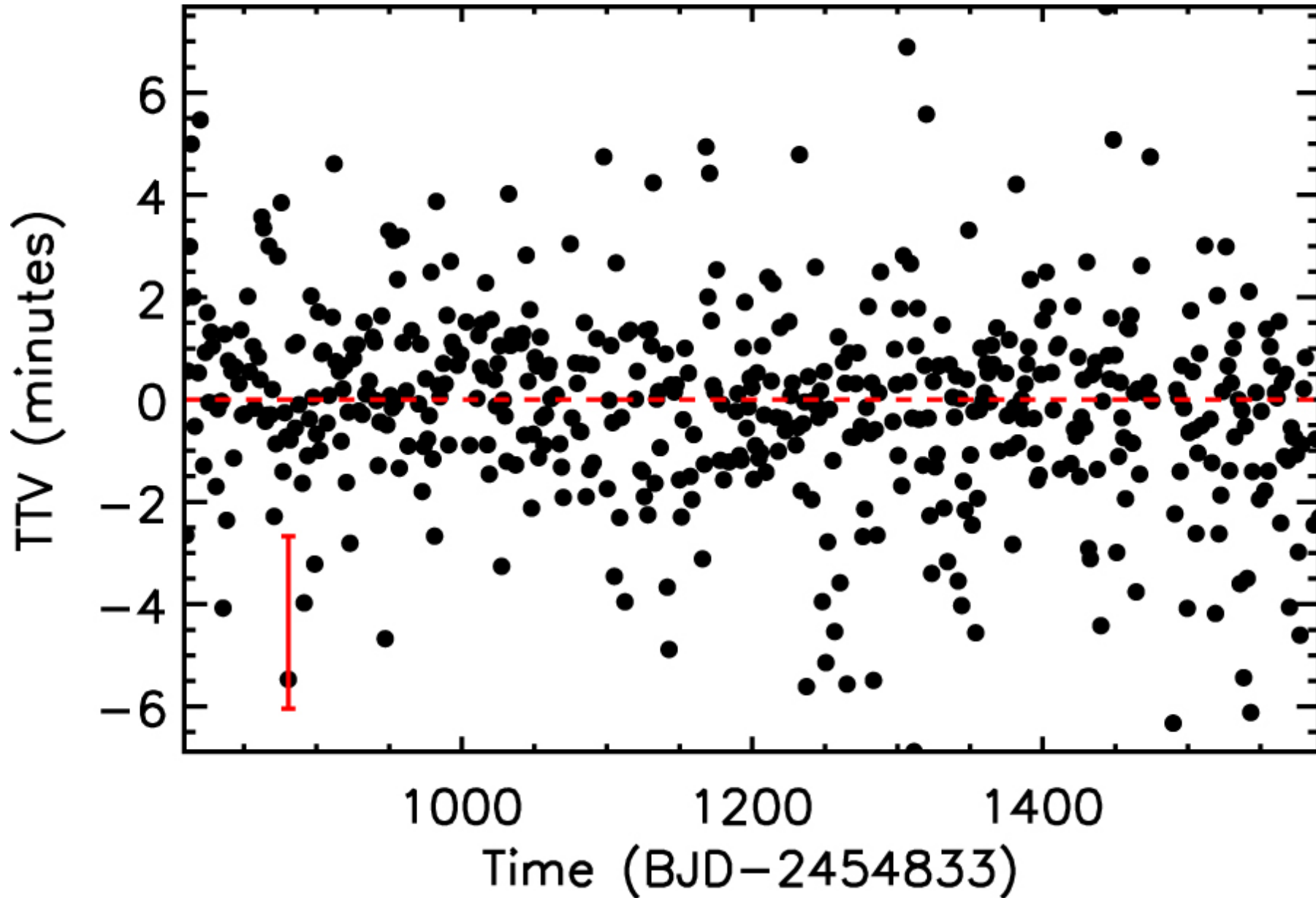
Figure 7. from The Gold Standard: Accurate Stellar and Planetary Parameters for Eight Kepler M Dwarf Systems Enabled by Parallaxes null 2017 AJ 153 267 doi:10.3847/1538-3881/aa7140 https://dx.doi.org/10.3847/1538-3881/aa7140 © 2017. The American Astronomical Society. All rights reserved.
