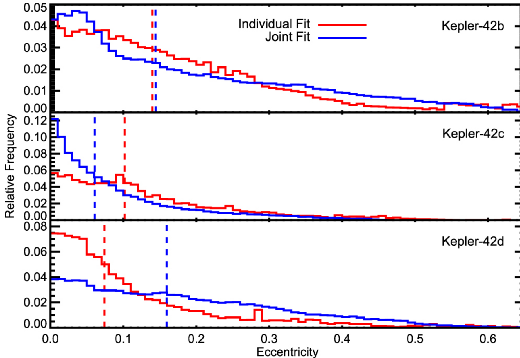
Figure 5. from The Gold Standard: Accurate Stellar and Planetary Parameters for Eight Kepler M Dwarf Systems Enabled by Parallaxes null 2017 AJ 153 267 doi:10.3847/1538-3881/aa7140 https://dx.doi.org/10.3847/1538-3881/aa7140 © 2017. The American Astronomical Society. All rights reserved.
