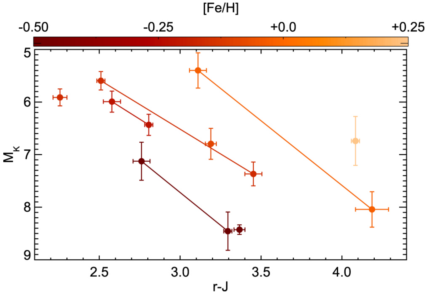
Figure 2. from The Gold Standard: Accurate Stellar and Planetary Parameters for Eight Kepler M Dwarf Systems Enabled by Parallaxes null 2017 AJ 153 267 doi:10.3847/1538-3881/aa7140 https://dx.doi.org/10.3847/1538-3881/aa7140 © 2017. The American Astronomical Society. All rights reserved.
