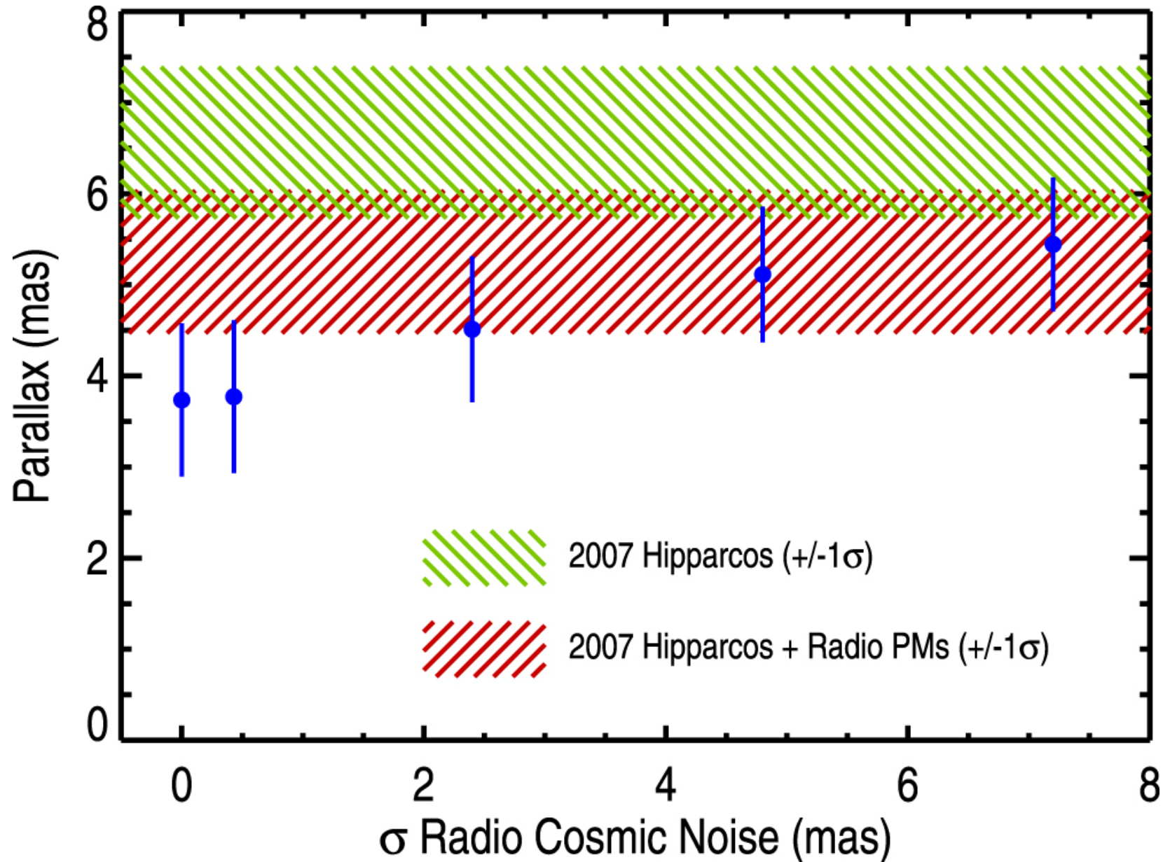
Figure 2. from An Updated 2017 Astrometric Solution for Betelgeuse null 2017 AJ 154 11 doi:10.3847/1538-3881/aa6ff9 https://dx.doi.org/10.3847/1538-3881/aa6ff9 © 2017. The American Astronomical Society. All rights reserved.
