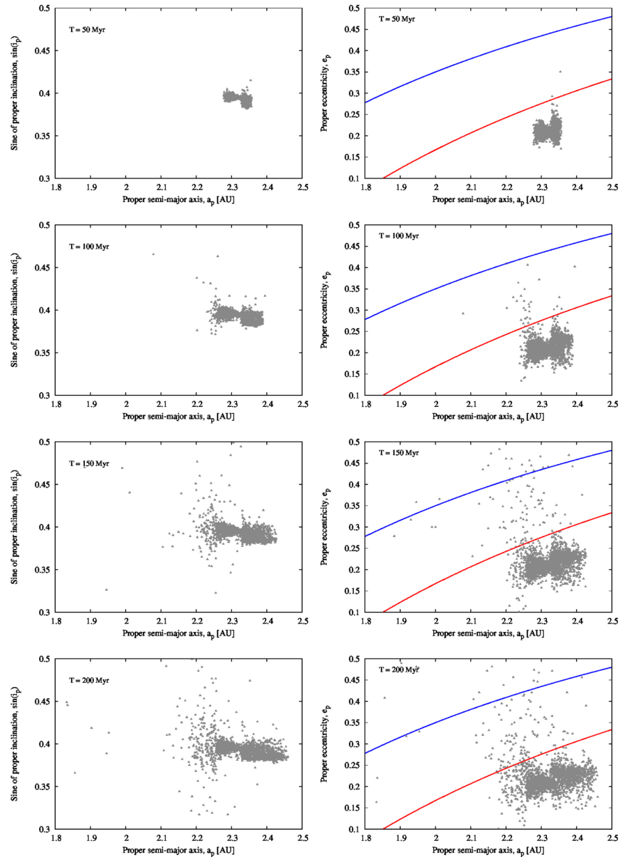
Figure 5. from A Dark Asteroid Family in the Phocaea Region null 2017 AJ 153 266 doi:10.3847/1538-3881/aa6ea8 https://dx.doi.org/10.3847/1538-3881/aa6ea8 © 2017. The American Astronomical Society. All rights reserved.
