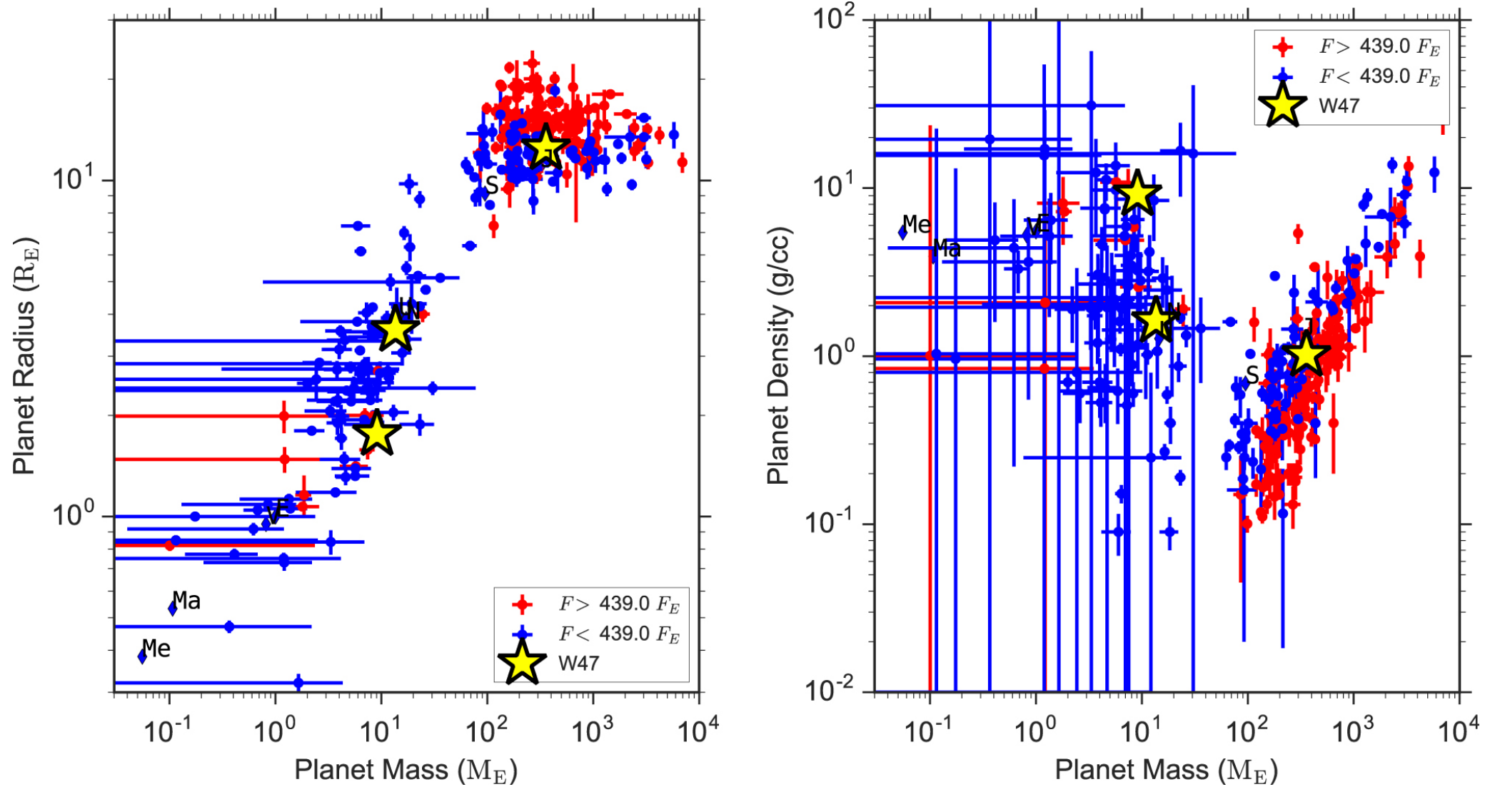
Figure 9. from New Insights on Planet Formation in WASP-47 from a Simultaneous Analysis of Radial Velocities and Transit Timing Variations null 2017 AJ 153 265 doi:10.3847/1538-3881/aa6c29 https://dx.doi.org/10.3847/1538-3881/aa6c29 © 2017. The American Astronomical Society. All rights reserved.
