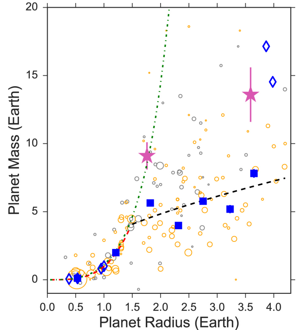
Figure 8. from New Insights on Planet Formation in WASP-47 from a Simultaneous Analysis of Radial Velocities and Transit Timing Variations null 2017 AJ 153 265 doi:10.3847/1538-3881/aa6c29 https://dx.doi.org/10.3847/1538-3881/aa6c29 © 2017. The American Astronomical Society. All rights reserved.
