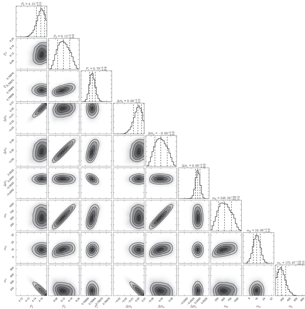
Figure 2. from New Insights on Planet Formation in WASP-47 from a Simultaneous Analysis of Radial Velocities and Transit Timing Variations null 2017 AJ 153 265 doi:10.3847/1538-3881/aa6c29 https://dx.doi.org/10.3847/1538-3881/aa6c29 © 2017. The American Astronomical Society. All rights reserved.
