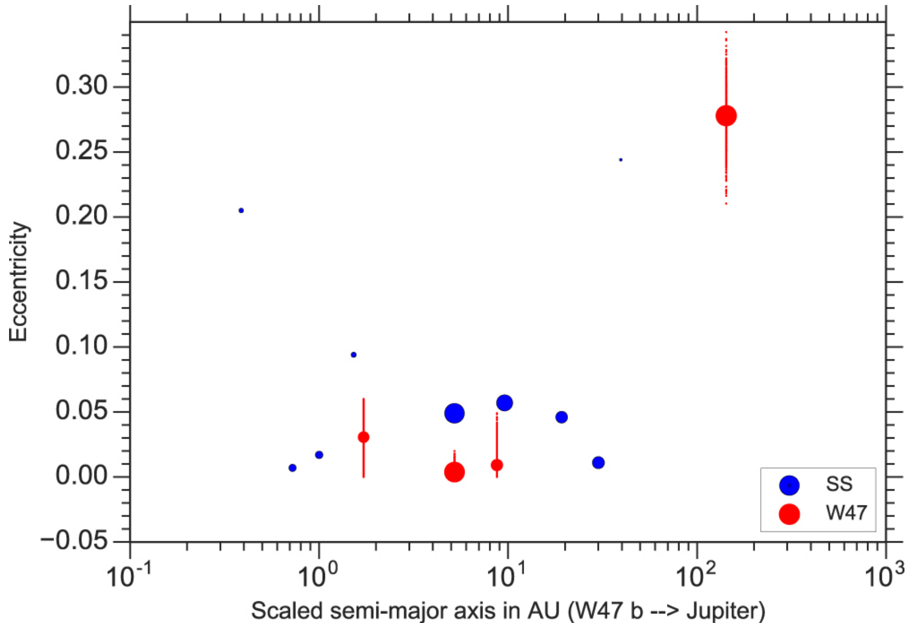
Figure 10. from New Insights on Planet Formation in WASP-47 from a Simultaneous Analysis of Radial Velocities and Transit Timing Variations null 2017 AJ 153 265 doi:10.3847/1538-3881/aa6c29 https://dx.doi.org/10.3847/1538-3881/aa6c29 © 2017. The American Astronomical Society. All rights reserved.
