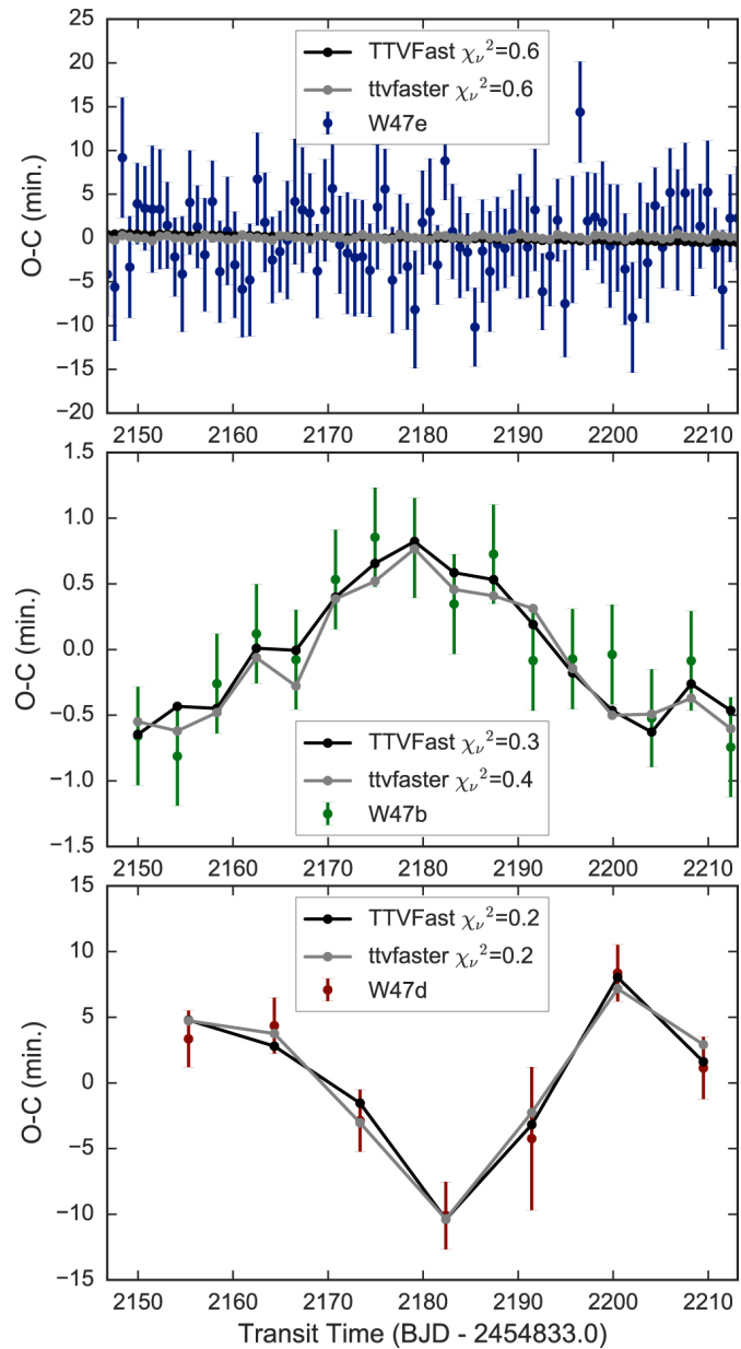
Figure 1. from New Insights on Planet Formation in WASP-47 from a Simultaneous Analysis of Radial Velocities and Transit Timing Variations null 2017 AJ 153 265 doi:10.3847/1538-3881/aa6c29 https://dx.doi.org/10.3847/1538-3881/aa6c29 © 2017. The American Astronomical Society. All rights reserved.
