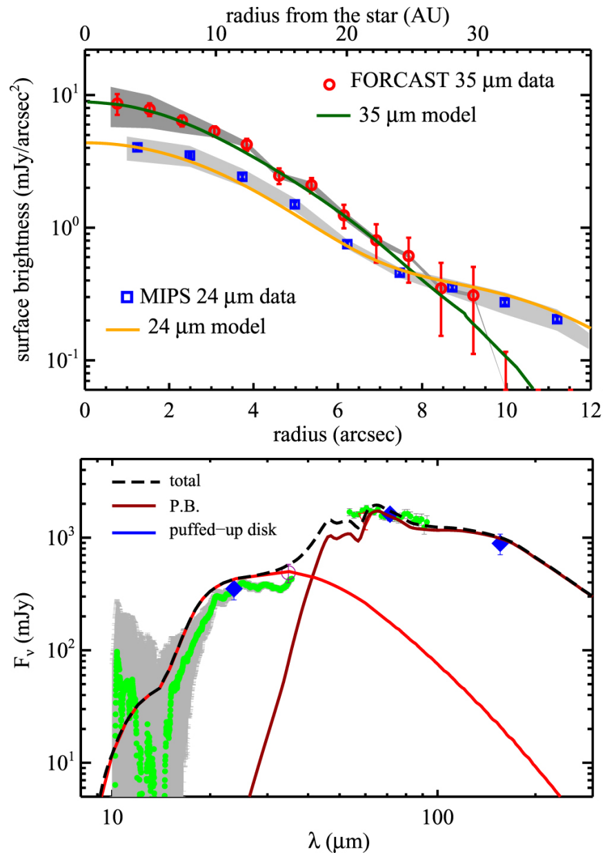
Figure 9. from The Inner 25 au Debris Distribution in the Eri System null 2017 AJ 153 226 doi:10.3847/1538-3881/aa696b https://dx.doi.org/10.3847/1538-3881/aa696b © 2017. The American Astronomical Society. All rights reserved.
