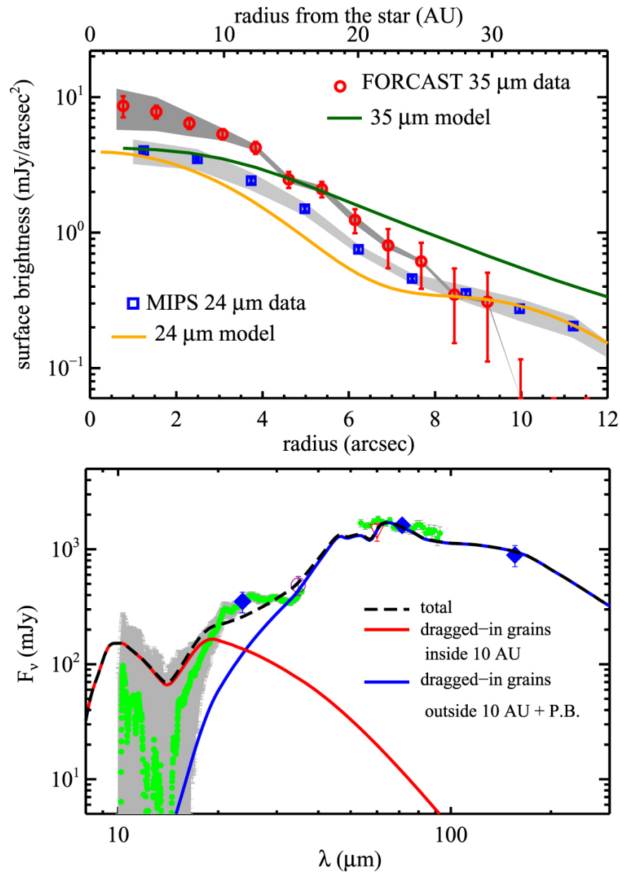
Figure 8. from The Inner 25 au Debris Distribution in the Eri System null 2017 AJ 153 226 doi:10.3847/1538-3881/aa696b https://dx.doi.org/10.3847/1538-3881/aa696b © 2017. The American Astronomical Society. All rights reserved.
