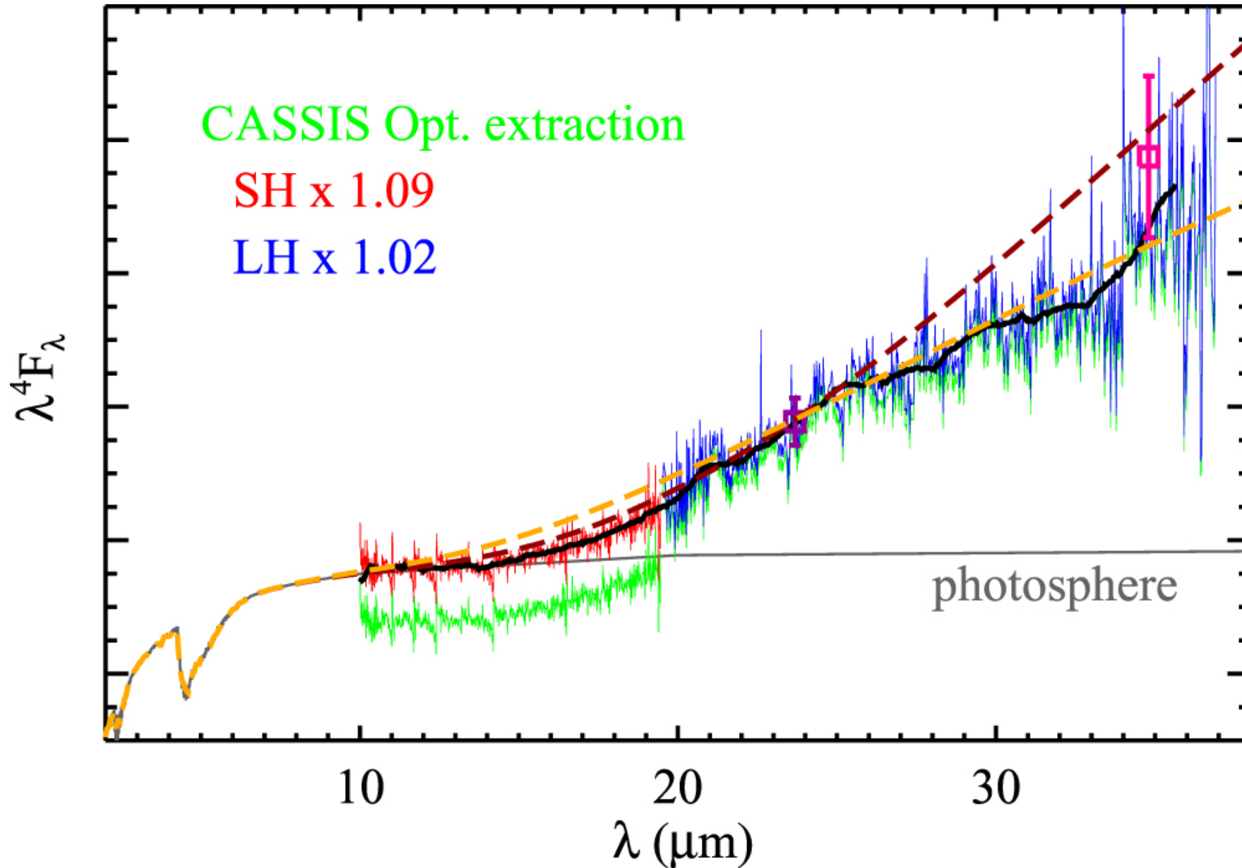
Figure 6. from The Inner 25 au Debris Distribution in the Eri System null 2017 AJ 153 226 doi:10.3847/1538-3881/aa696b https://dx.doi.org/10.3847/1538-3881/aa696b © 2017. The American Astronomical Society. All rights reserved.
