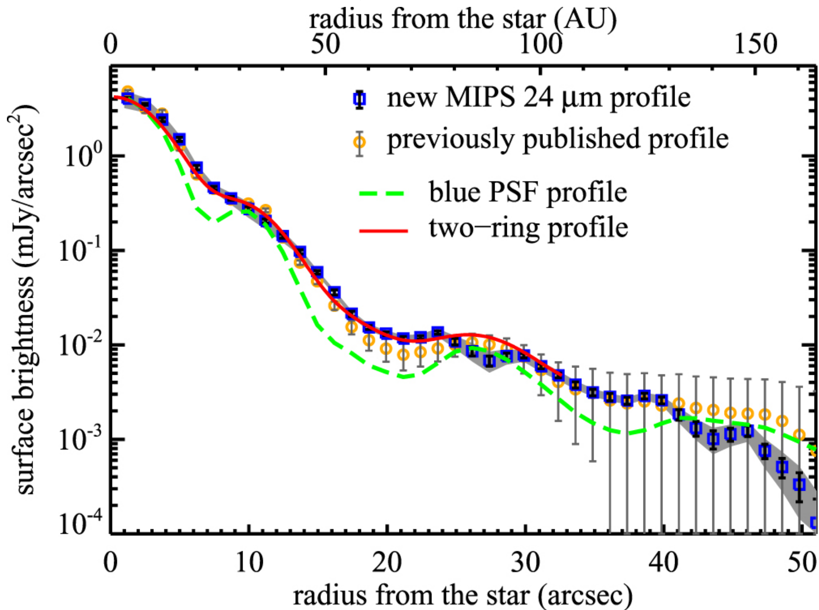
Figure 5. from The Inner 25 au Debris Distribution in the Eri System null 2017 AJ 153 226 doi:10.3847/1538-3881/aa696b https://dx.doi.org/10.3847/1538-3881/aa696b © 2017. The American Astronomical Society. All rights reserved.
