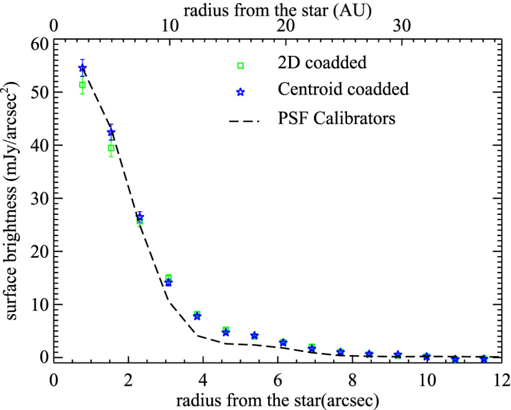
Figure 2. from The Inner 25 au Debris Distribution in the Eri System null 2017 AJ 153 226 doi:10.3847/1538-3881/aa696b https://dx.doi.org/10.3847/1538-3881/aa696b © 2017. The American Astronomical Society. All rights reserved.
