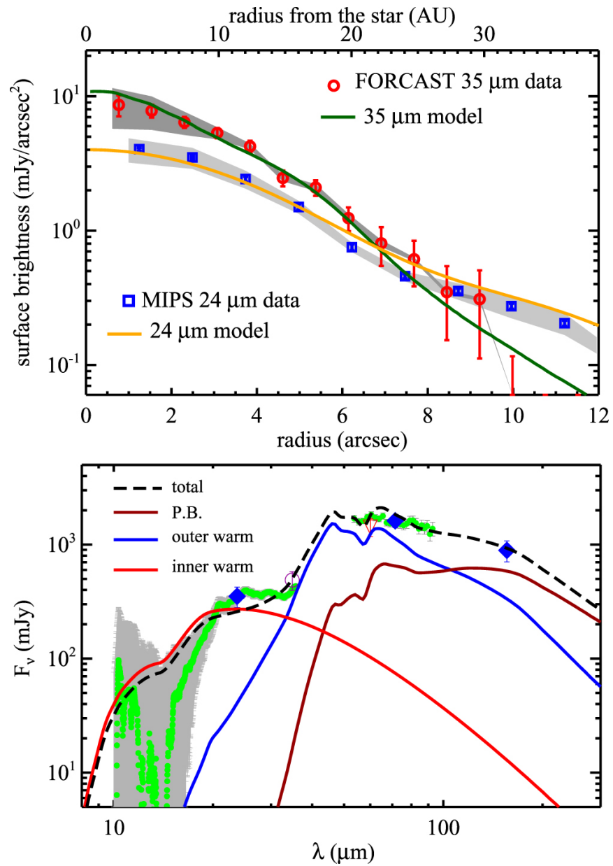
Figure 10. from The Inner 25 au Debris Distribution in the Eri System null 2017 AJ 153 226 doi:10.3847/1538-3881/aa696b https://dx.doi.org/10.3847/1538-3881/aa696b © 2017. The American Astronomical Society. All rights reserved.
