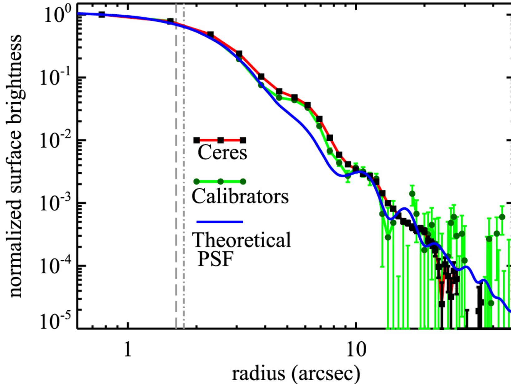
Figure 1. from The Inner 25 au Debris Distribution in the Eri System null 2017 AJ 153 226 doi:10.3847/1538-3881/aa696b https://dx.doi.org/10.3847/1538-3881/aa696b © 2017. The American Astronomical Society. All rights reserved.
