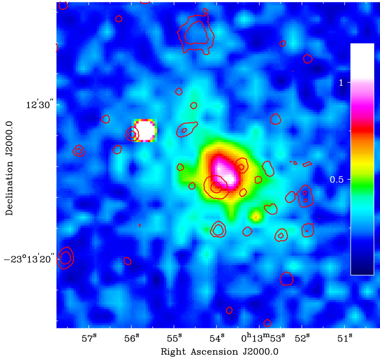
Figure 6. from CHANDRA AND VERY LARGE ARRAY OBSERVATIONS OF THE NEARBY Sd GALAXY NGC 45 null 2015 AJ 150 91 doi:10.1088/0004-6256/150/3/91 https://dx.doi.org/10.1088/0004-6256/150/3/91 © 2015. The American Astronomical Society. All rights reserved.
