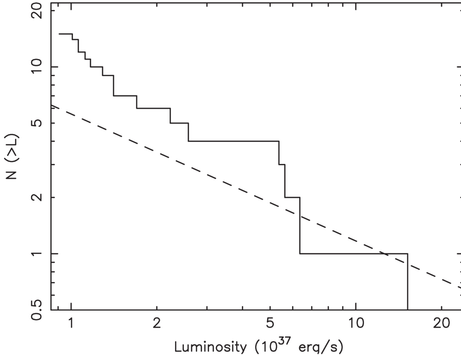
Figure 5. from CHANDRA AND VERY LARGE ARRAY OBSERVATIONS OF THE NEARBY Sd GALAXY NGC 45 null 2015 AJ 150 91 doi:10.1088/0004-6256/150/3/91 https://dx.doi.org/10.1088/0004-6256/150/3/91 © 2015. The American Astronomical Society. All rights reserved.
