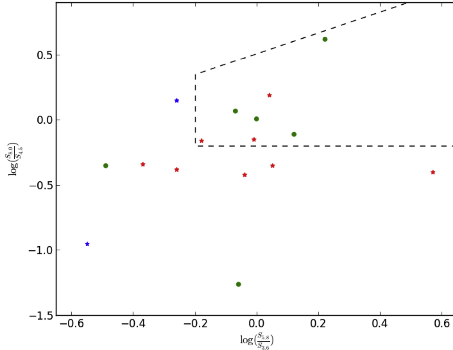
Figure 4. from CHANDRA AND VERY LARGE ARRAY OBSERVATIONS OF THE NEARBY Sd GALAXY NGC 45 null 2015 AJ 150 91 doi:10.1088/0004-6256/150/3/91 https://dx.doi.org/10.1088/0004-6256/150/3/91 © 2015. The American Astronomical Society. All rights reserved.
