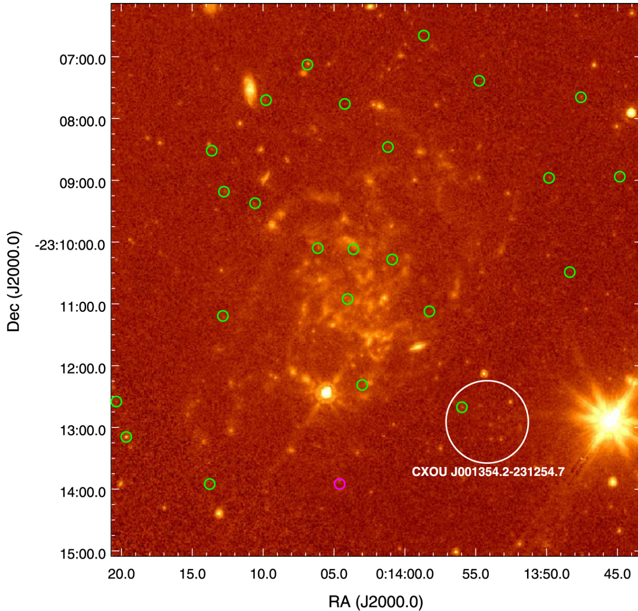
Figure 1. from CHANDRA AND VERY LARGE ARRAY OBSERVATIONS OF THE NEARBY Sd GALAXY NGC 45 null 2015 AJ 150 91 doi:10.1088/0004-6256/150/3/91 https://dx.doi.org/10.1088/0004-6256/150/3/91 © 2015. The American Astronomical Society. All rights reserved.
