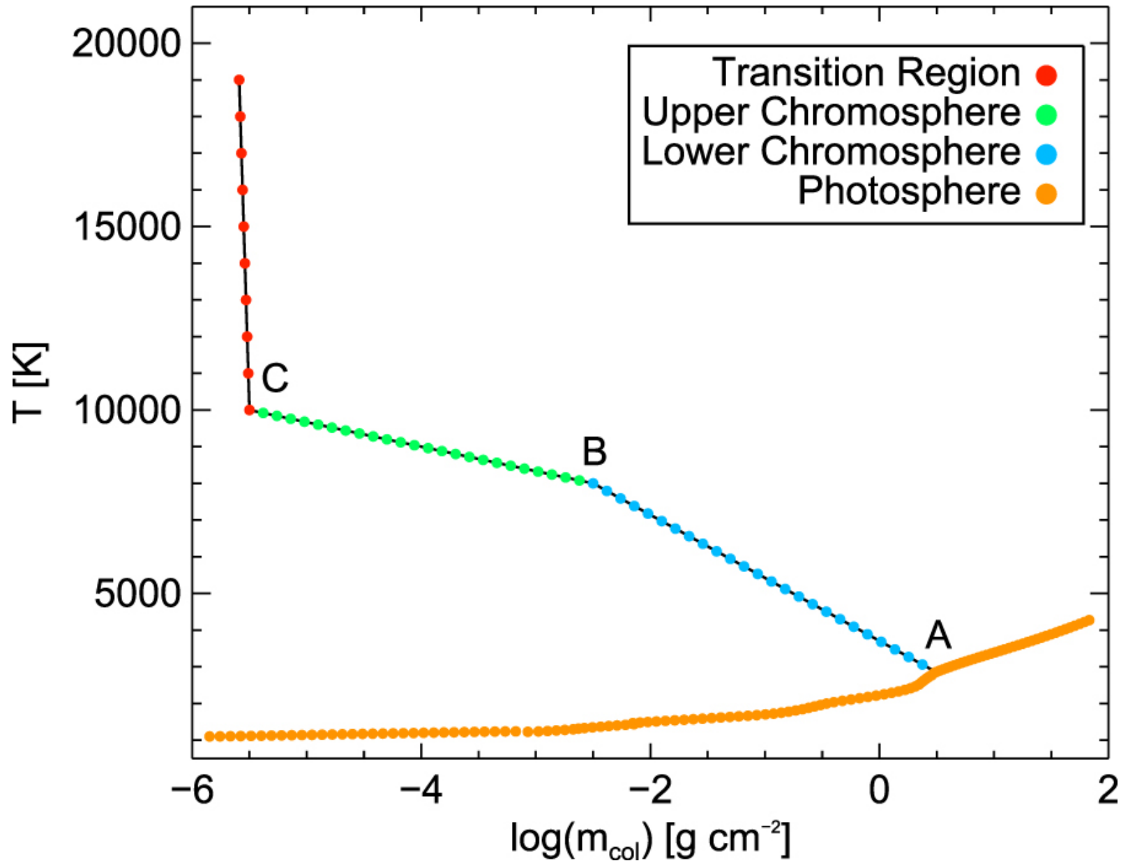
Figure 8. from BOSS ULTRACOOOL DWARFS. I. COLORS AND MAGNETIC ACTIVITY OF M AND L DWARFS null 2015 AJ 149 158 doi:10.1088/0004-6256/149/5/158 https://dx.doi.org/10.1088/0004-6256/149/5/158 © 2015. The American Astronomical Society. All rights reserved.
