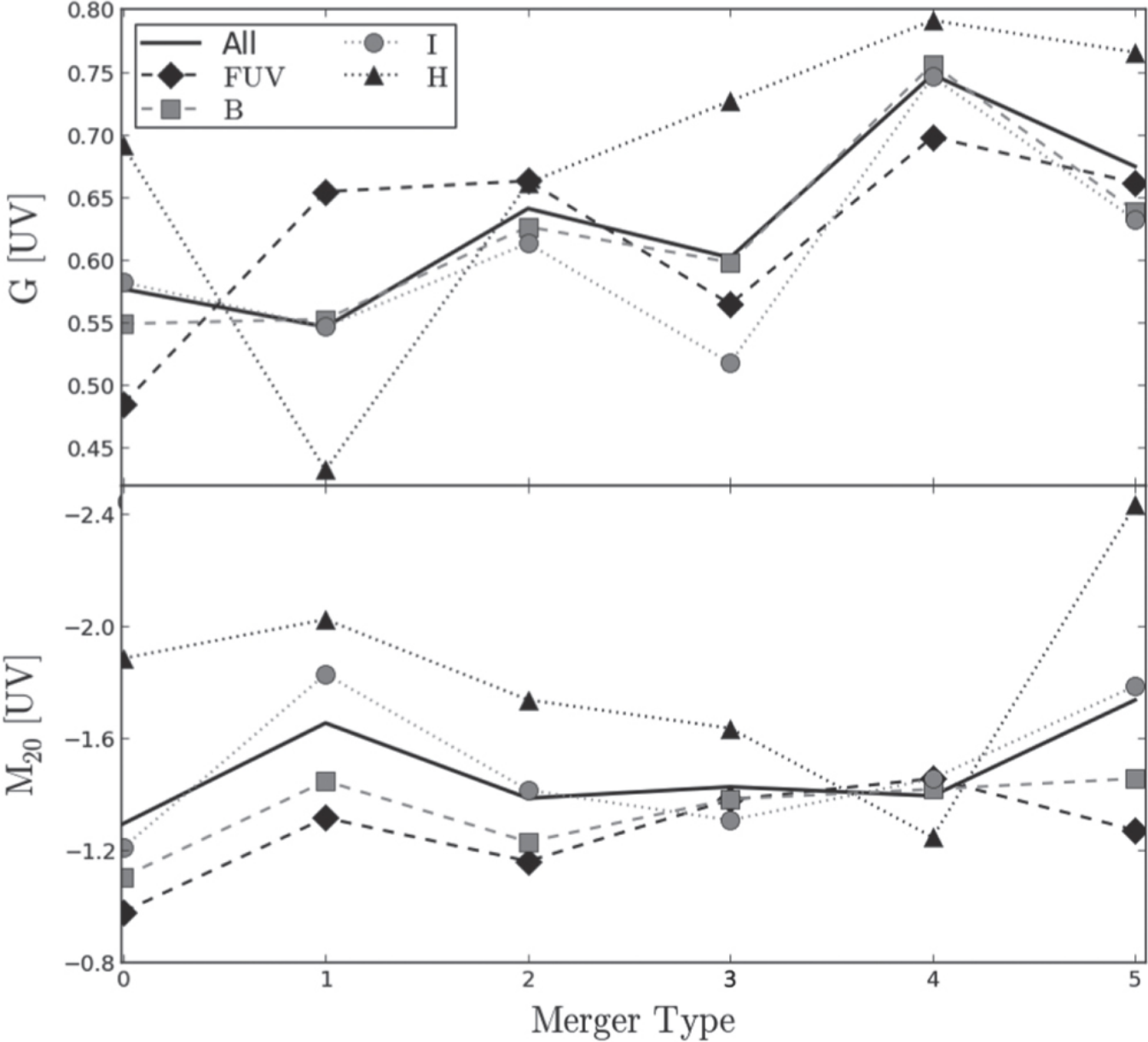
Figure 3. from THE FUV TO NEAR-IR MORPHOLOGIES OF LUMINOUS INFRARED GALAXIES IN THE GOALS SAMPLE null 2014 AJ 148 111 doi:10.1088/0004-6256/148/6/111 https://dx.doi.org/10.1088/0004-6256/148/6/111 © 2014. The American Astronomical Society. All rights reserved.
