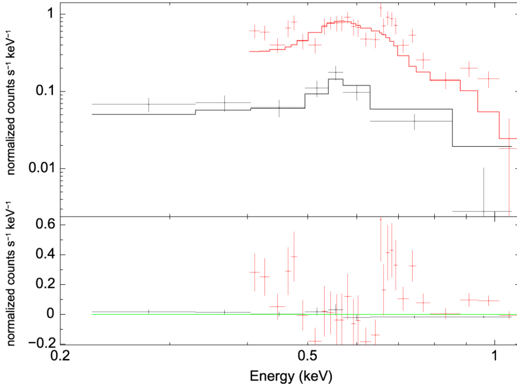
Figure 7. from DIFFUSE X-RAY EMISSION FROM THE SUPERBUBBLES N70 AND N185 IN THE LARGE MAGELLANIC CLOUD null 2014 AJ 148 102 doi:10.1088/0004-6256/148/5/102 https://dx.doi.org/10.1088/0004-6256/148/5/102 © 2014. The American Astronomical Society. All rights reserved.
