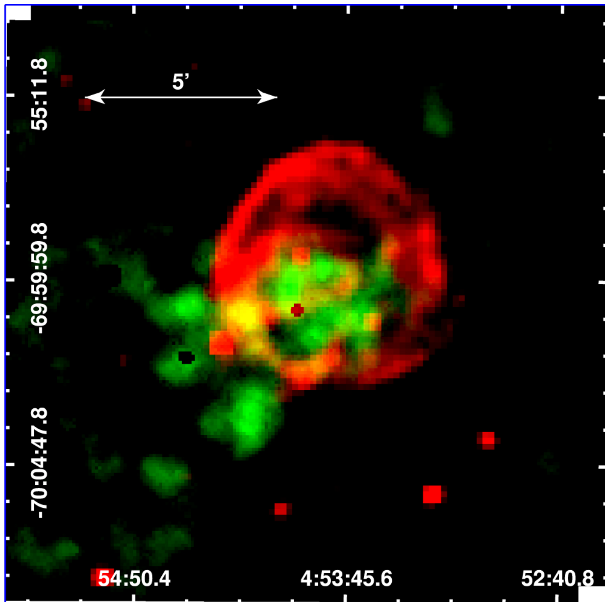
Figure 6. from DIFFUSE X-RAY EMISSION FROM THE SUPERBUBBLES N70 AND N185 IN THE LARGE MAGELLANIC CLOUD null 2014 AJ 148 102 doi:10.1088/0004-6256/148/5/102 https://dx.doi.org/10.1088/0004-6256/148/5/102 © 2014. The American Astronomical Society. All rights reserved.
