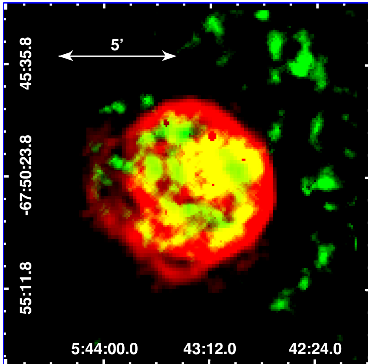
Figure 3. from DIFFUSE X-RAY EMISSION FROM THE SUPERBUBBLES N70 AND N185 IN THE LARGE MAGELLANIC CLOUD null 2014 AJ 148 102 doi:10.1088/0004-6256/148/5/102 https://dx.doi.org/10.1088/0004-6256/148/5/102 © 2014. The American Astronomical Society. All rights reserved.
