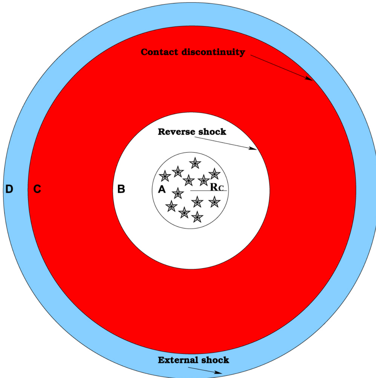
Figure 1. from DIFFUSE X-RAY EMISSION FROM THE SUPERBUBBLES N70 AND N185 IN THE LARGE MAGELLANIC CLOUD null 2014 AJ 148 102 doi:10.1088/0004-6256/148/5/102 https://dx.doi.org/10.1088/0004-6256/148/5/102 © 2014. The American Astronomical Society. All rights reserved.
