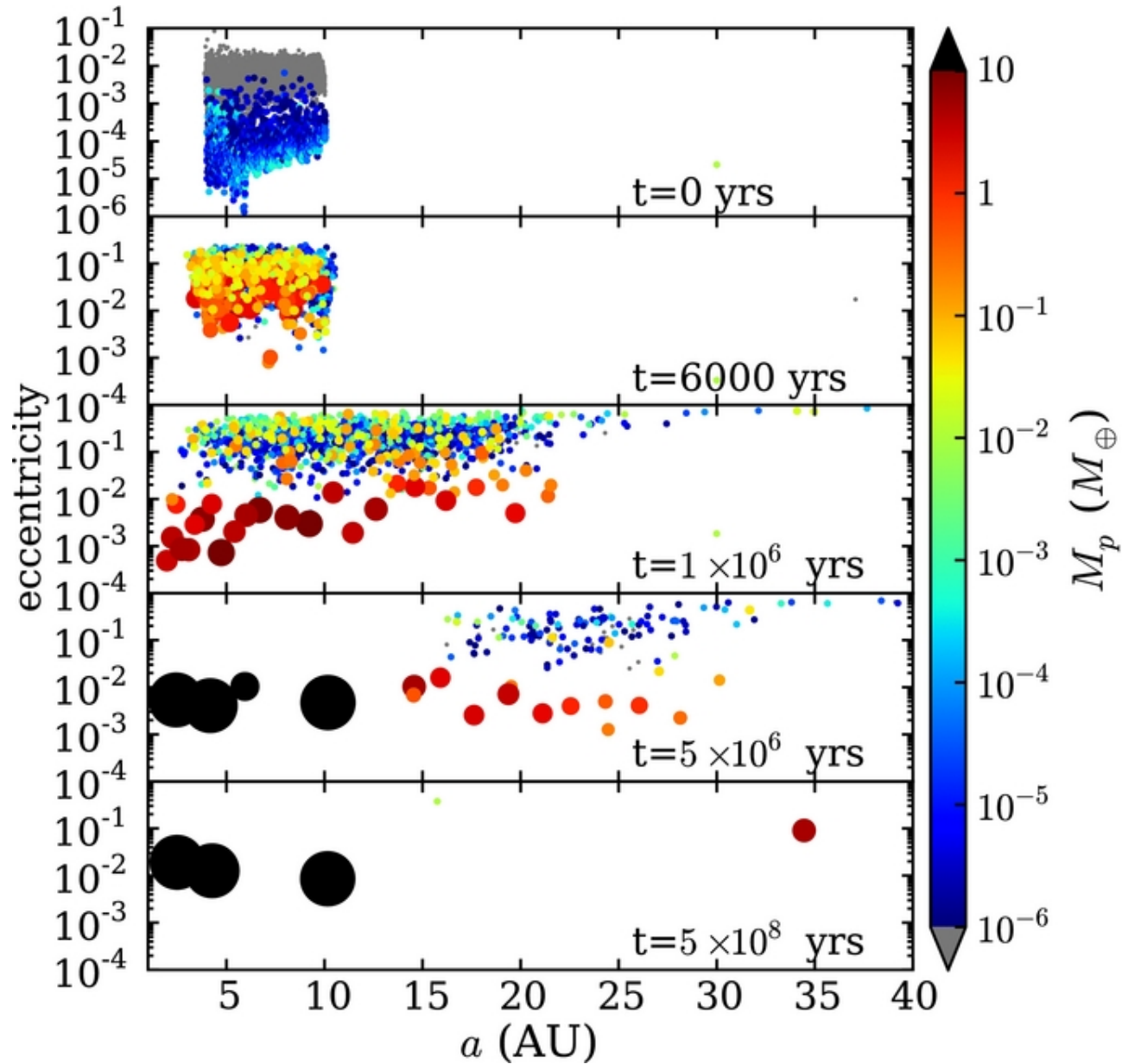
Figure 6. from Challenges in Forming the Solar System's Giant Planet Cores via Pebble Accretion Kretke & Levison 2014 AJ 148 109 doi:10.1088/0004-6256/148/6/109 https://dx.doi.org/10.1088/0004-6256/148/6/109 © 2014. The American Astronomical Society. All rights reserved.
