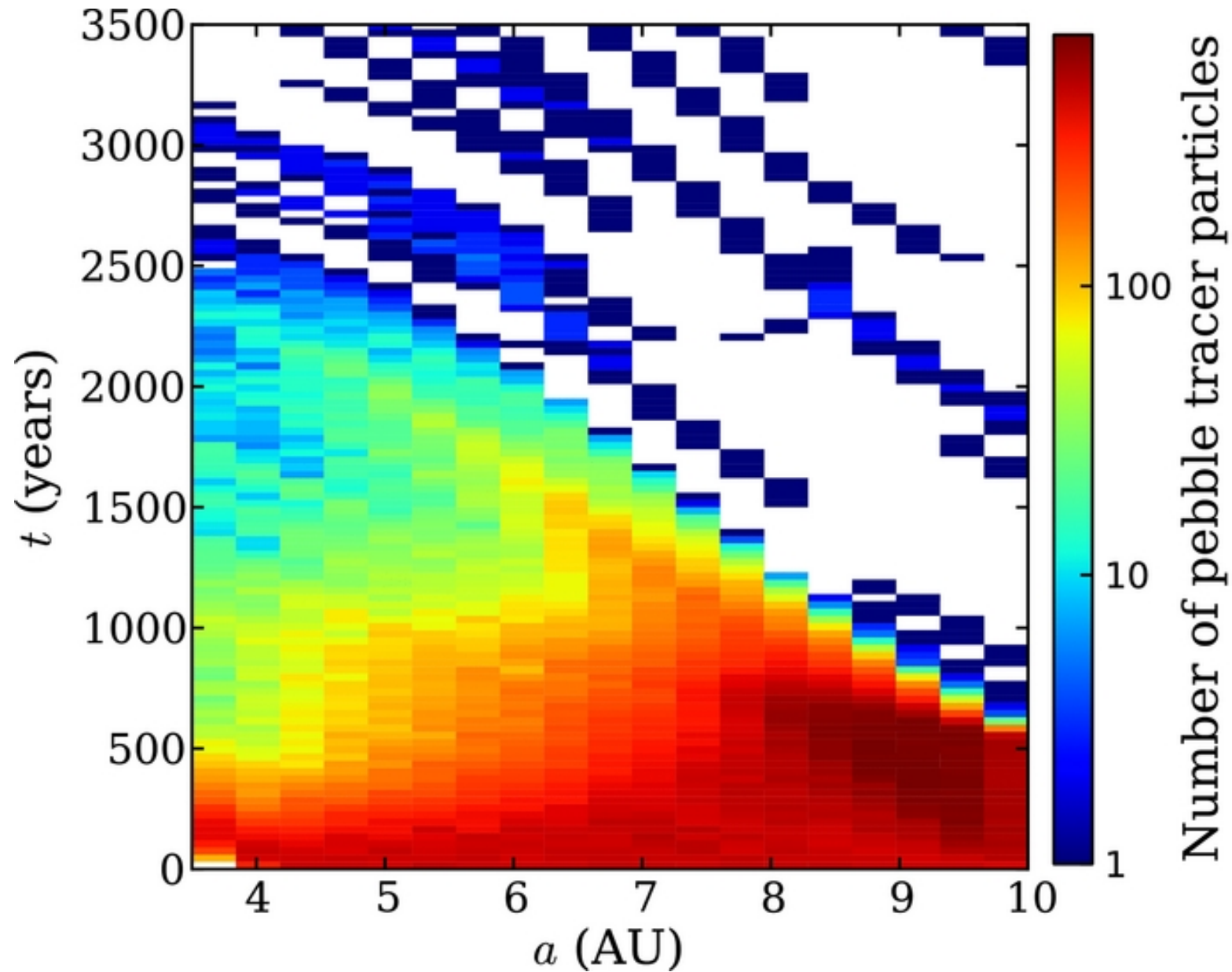
Figure 4. from Challenges in Forming the Solar System's Giant Planet Cores via Pebble Accretion Kretke & Levison 2014 AJ 148 109 doi:10.1088/0004-6256/148/6/109 https://dx.doi.org/10.1088/0004-6256/148/6/109 © 2014. The American Astronomical Society. All rights reserved.
