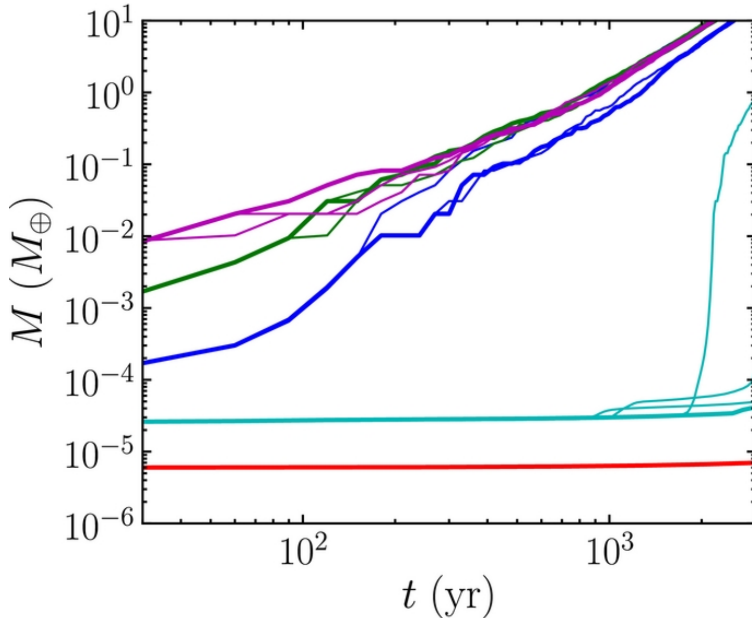
Figure 2. from Challenges in Forming the Solar System's Giant Planet Cores via Pebble Accretion Kretke & Levison 2014 AJ 148 109 doi:10.1088/0004-6256/148/6/109 https://dx.doi.org/10.1088/0004-6256/148/6/109 © 2014. The American Astronomical Society. All rights reserved.
