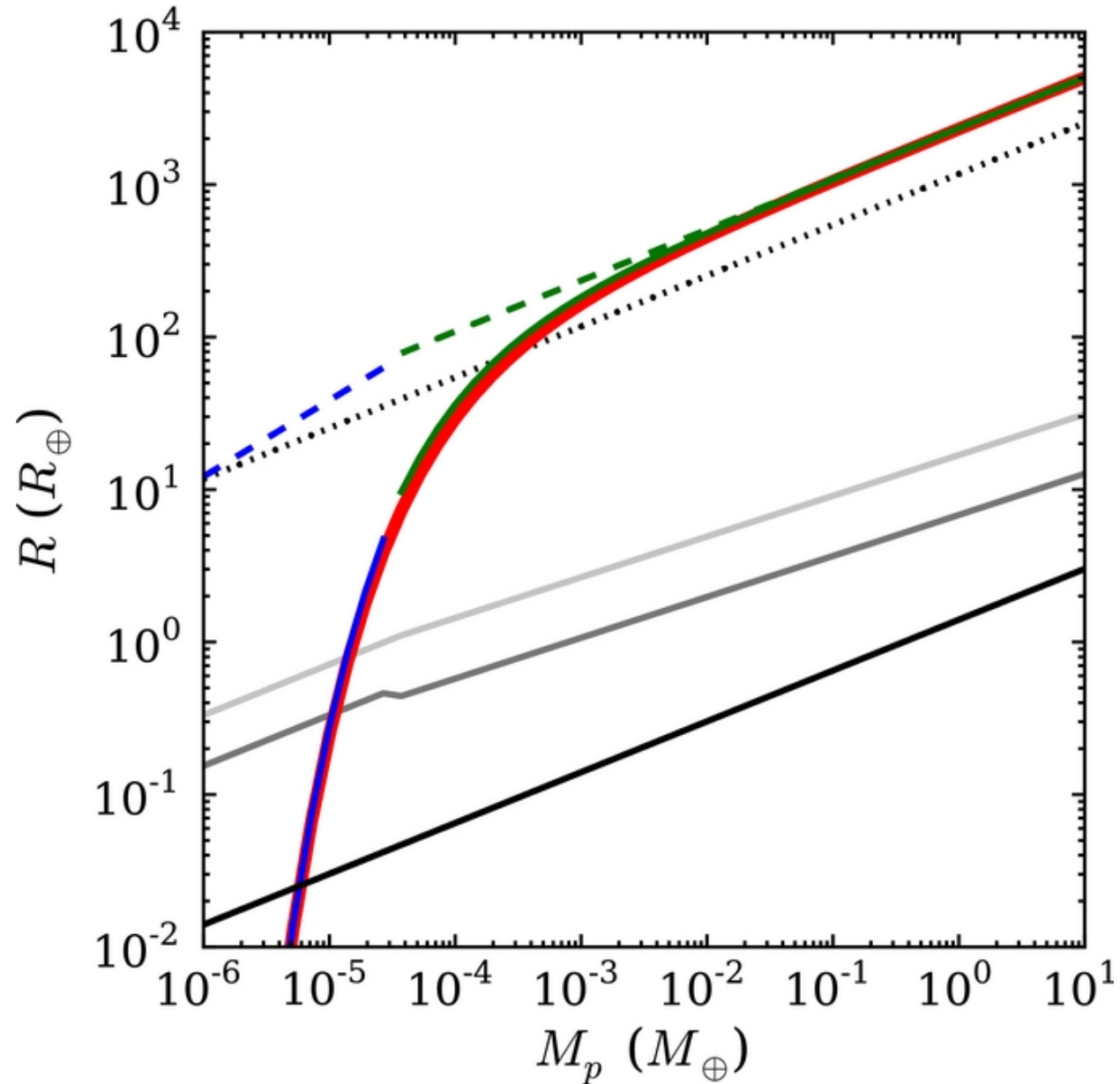
Figure 1. from Challenges in Forming the Solar System's Giant Planet Cores via Pebble Accretion Kretke & Levison 2014 AJ 148 109 doi:10.1088/0004-6256/148/6/109 https://dx.doi.org/10.1088/0004-6256/148/6/109 © 2014. The American Astronomical Society. All rights reserved.
