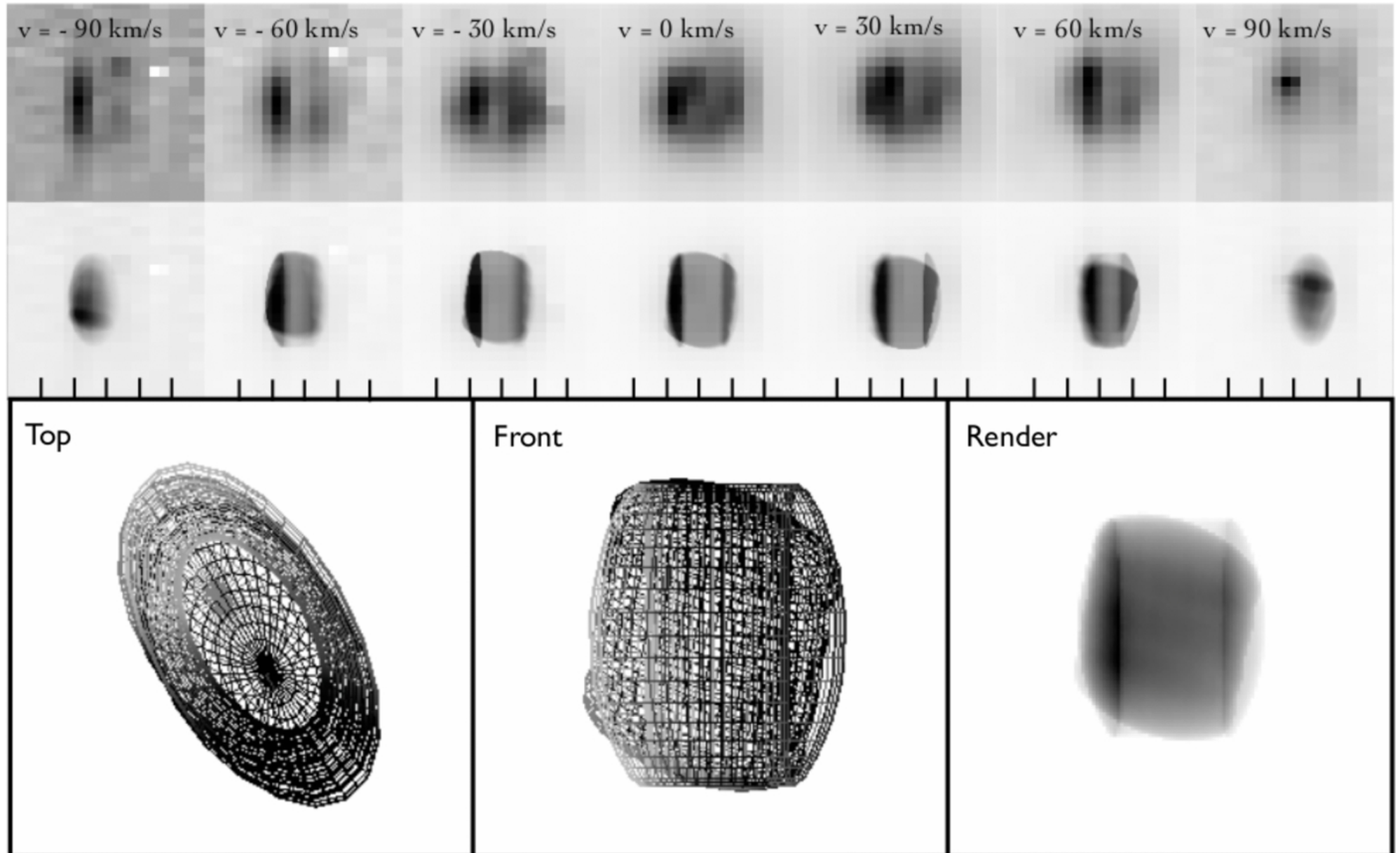
Figure 8. from A Detailed Study of the Structure of the Nested Planetary Nebula, Hb 12, the Matryoshka Nebula Clark et al. 2014 AJ 148 98 doi:10.1088/0004-6256/148/5/98 https://dx.doi.org/10.1088/0004-6256/148/5/98 © 2014. The American Astronomical Society. All rights reserved.
