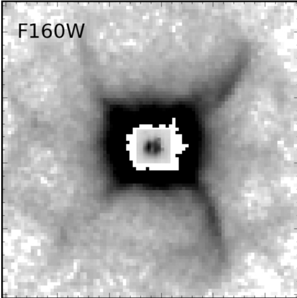
Figure 7. from A Detailed Study of the Structure of the Nested Planetary Nebula, Hb 12, the Matryoshka Nebula Clark et al. 2014 AJ 148 98 doi:10.1088/0004-6256/148/5/98 https://dx.doi.org/10.1088/0004-6256/148/5/98 © 2014. The American Astronomical Society. All rights reserved.
