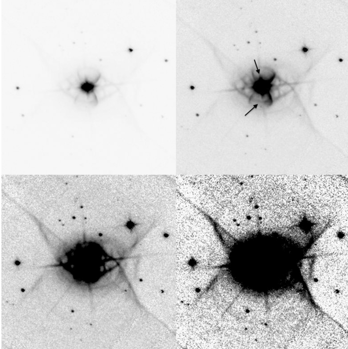
Figure 3. from A Detailed Study of the Structure of the Nested Planetary Nebula, Hb 12, the Matryoshka Nebula Clark et al. 2014 AJ 148 98 doi:10.1088/0004-6256/148/5/98 https://dx.doi.org/10.1088/0004-6256/148/5/98 © 2014. The American Astronomical Society. All rights reserved.
