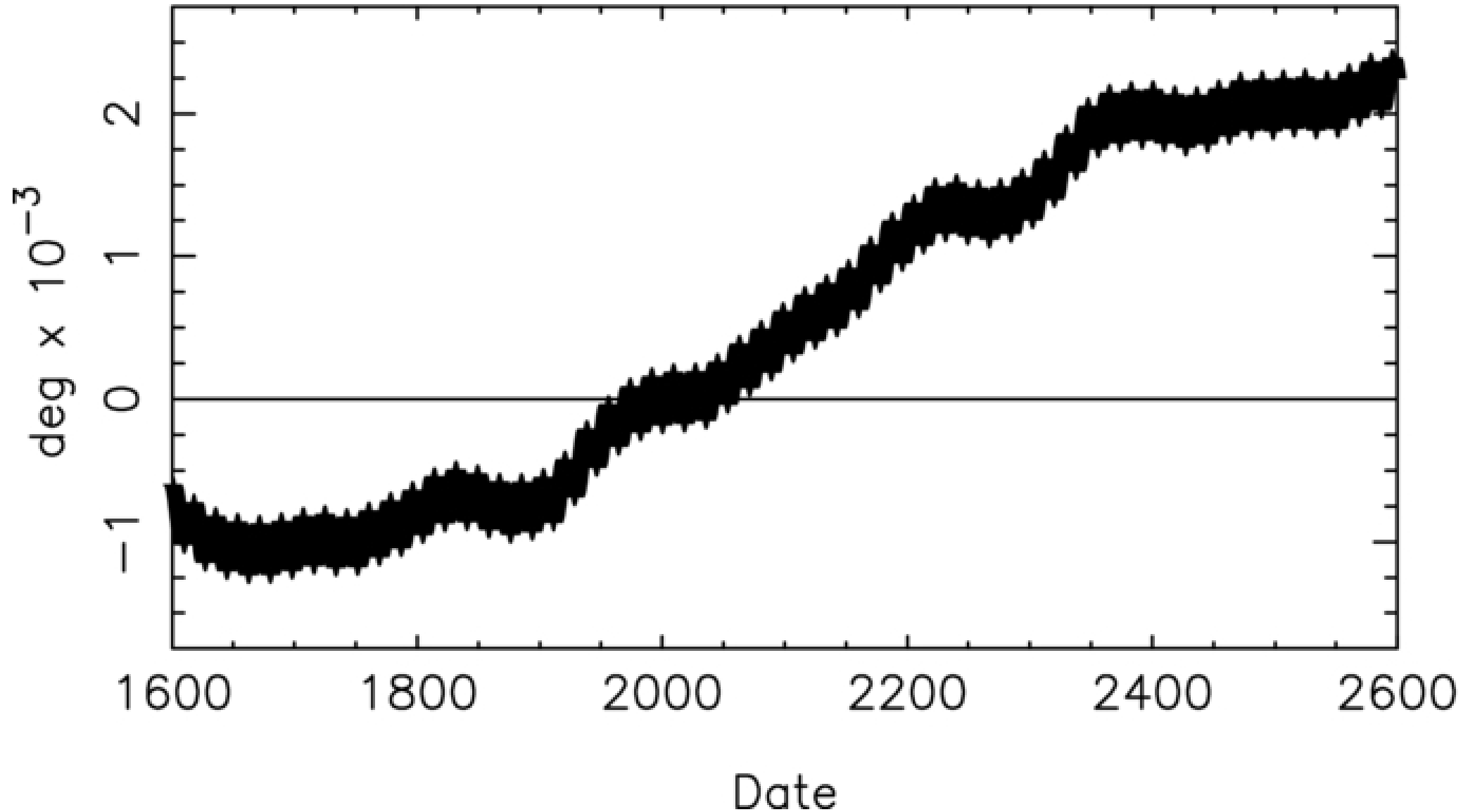
Figure 2. from The Orbits of the Uranian Satellites and Rings, the Gravity Field of the Uranian System, and the Orientation of the Pole of Uranus Jacobson 2014 AJ 148 76 doi:10.1088/0004-6256/148/5/76 https://dx.doi.org/10.1088/0004-6256/148/5/76 © 2014. The American Astronomical Society. All rights reserved.
