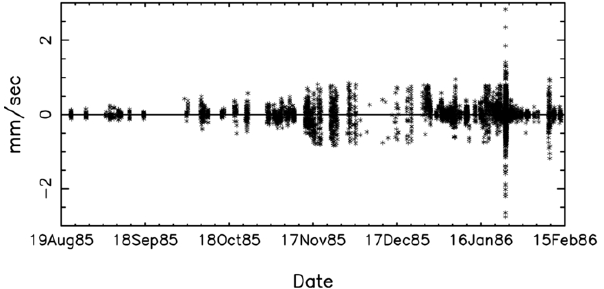
Figure 1. from The Orbits of the Uranian Satellites and Rings, the Gravity Field of the Uranian System, and the Orientation of the Pole of Uranus Jacobson 2014 AJ 148 76 doi:10.1088/0004-6256/148/5/76 https://dx.doi.org/10.1088/0004-6256/148/5/76 © 2014. The American Astronomical Society. All rights reserved.
