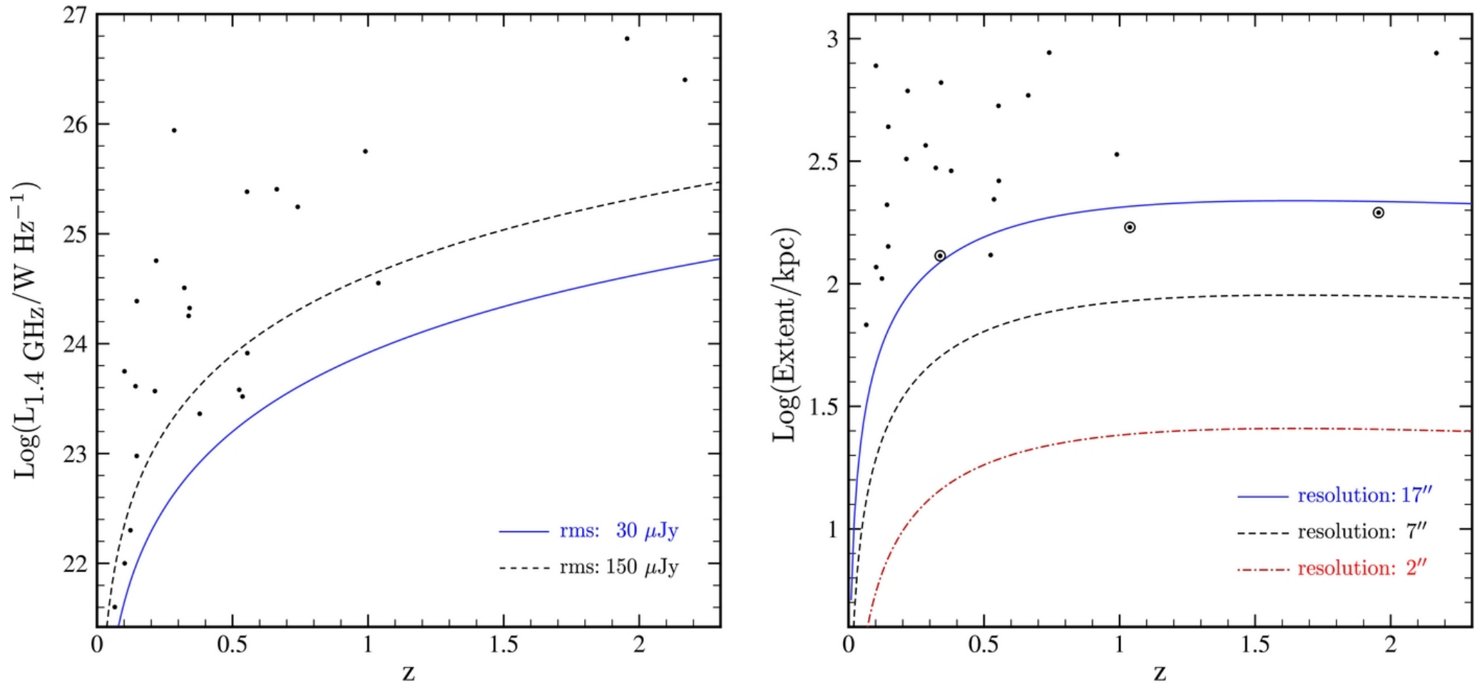
Figure 5. from Bent-tailed Radio Sources in the Australia Telescope Large Area Survey of the Chandra Deep Field South Dehghan et al. 2014 AJ 148 75 doi:10.1088/0004-6256/148/5/75 https://dx.doi.org/10.1088/0004-6256/148/5/75 © 2014. The American Astronomical Society. All rights reserved.
