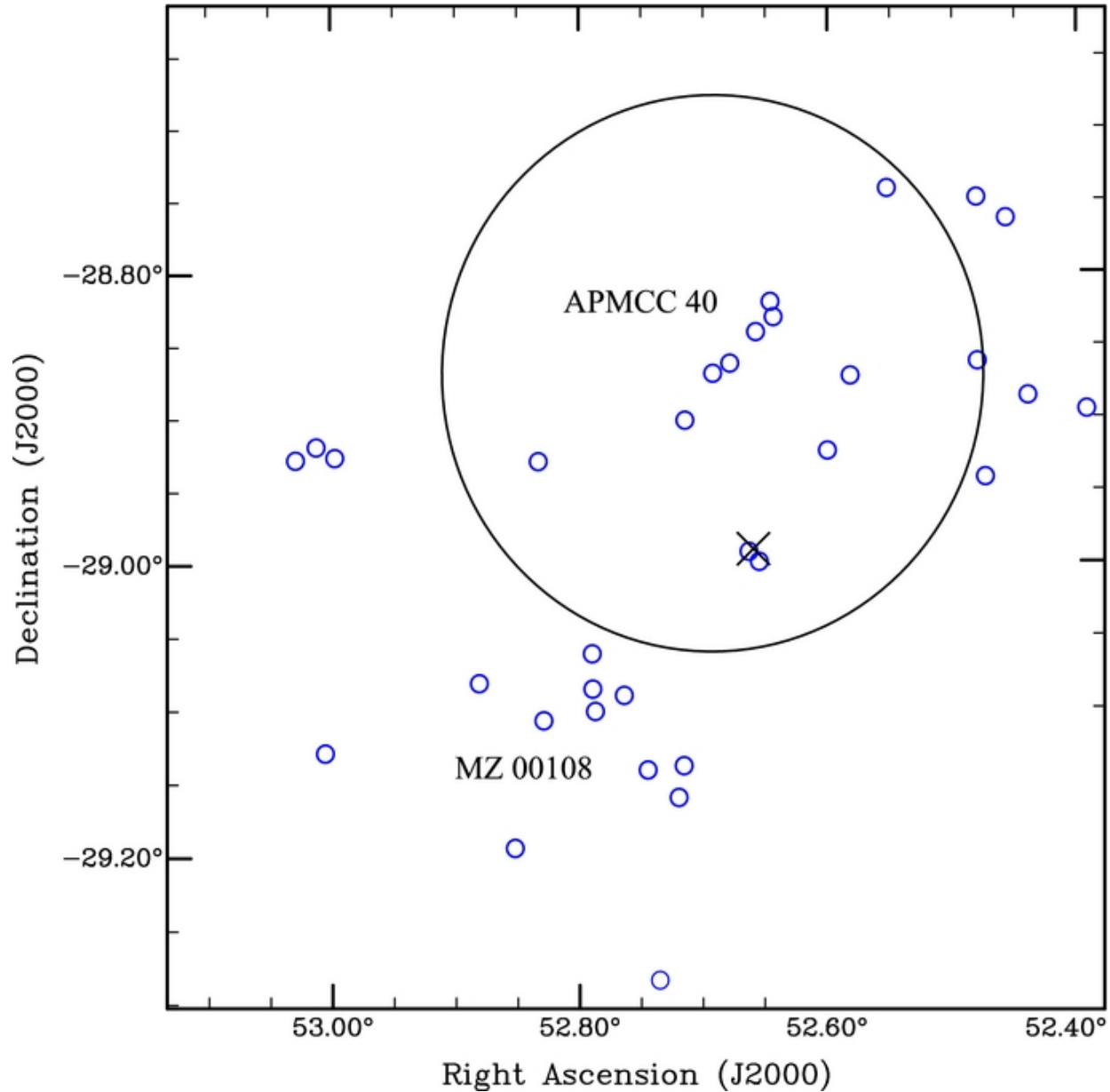
Figure 4. from Bent-tailed Radio Sources in the Australia Telescope Large Area Survey of the Chandra Deep Field South Dehghan et al. 2014 AJ 148 75 doi:10.1088/0004-6256/148/5/75 https://dx.doi.org/10.1088/0004-6256/148/5/75 © 2014. The American Astronomical Society. All rights reserved.
