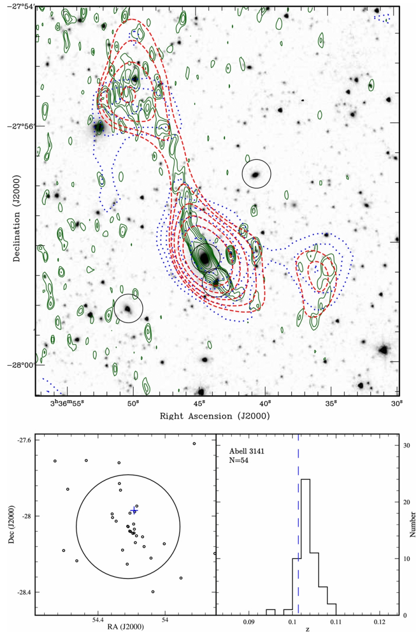
Figure 3. from Bent-tailed Radio Sources in the Australia Telescope Large Area Survey of the Chandra Deep Field South Dehghan et al. 2014 AJ 148 75 doi:10.1088/0004-6256/148/5/75 https://dx.doi.org/10.1088/0004-6256/148/5/75 © 2014. The American Astronomical Society. All rights reserved.
