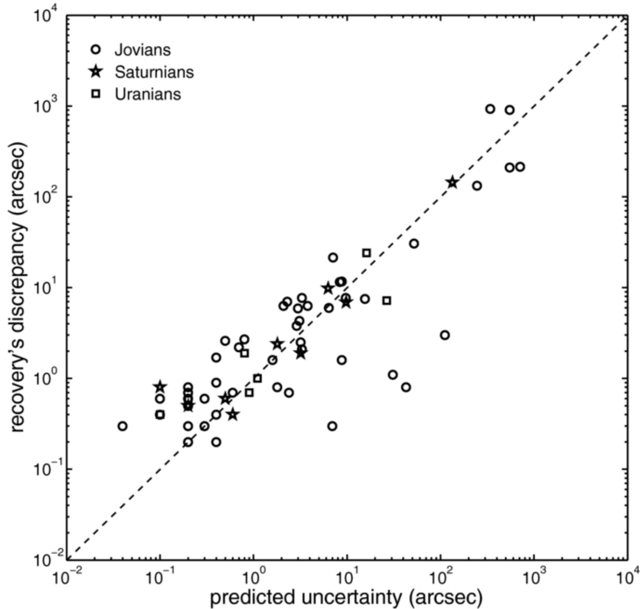
Figure 2. from Irregular Satellites of the Outer Planets: Orbital Uncertainties and Astrometric Recoveries in 2009–2011 Jacobson et al. 2012 AJ 144 132 doi:10.1088/0004-6256/144/5/132 http://dx.doi.org/10.1088/0004-6256/144/5/132 © 2012. The American Astronomical Society. All rights reserved.
