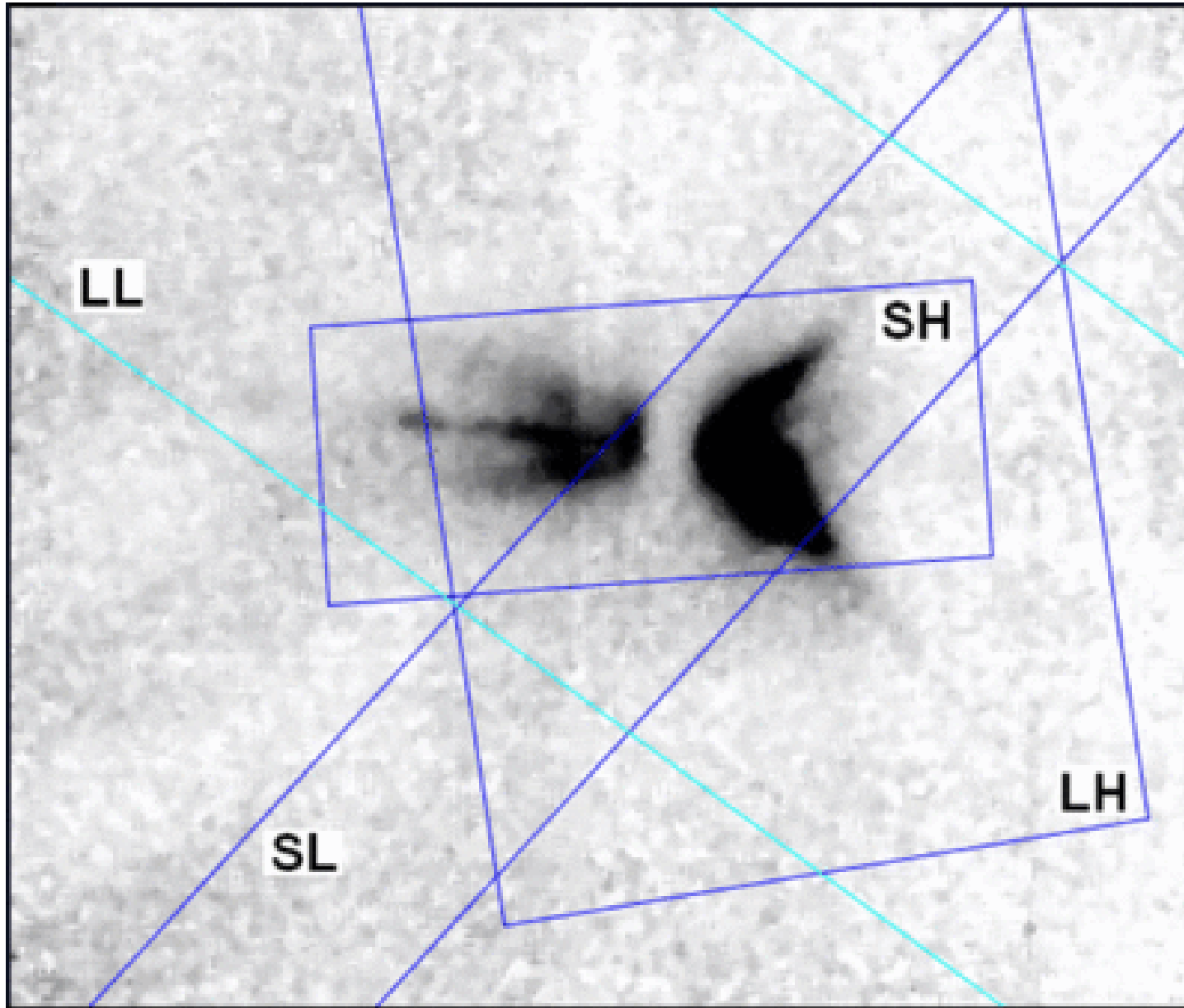
Fig. 1. from Spitzer IRS Spectra and Envelope Models of Class I Protostars in Taurus Furlan et al. 2008 ApJS 176 184 doi:10.1086/527301 https://dx.doi.org/10.1086/527301 © 2008. The American Astronomical Society. All rights reserved. Printed in U.S.A.
