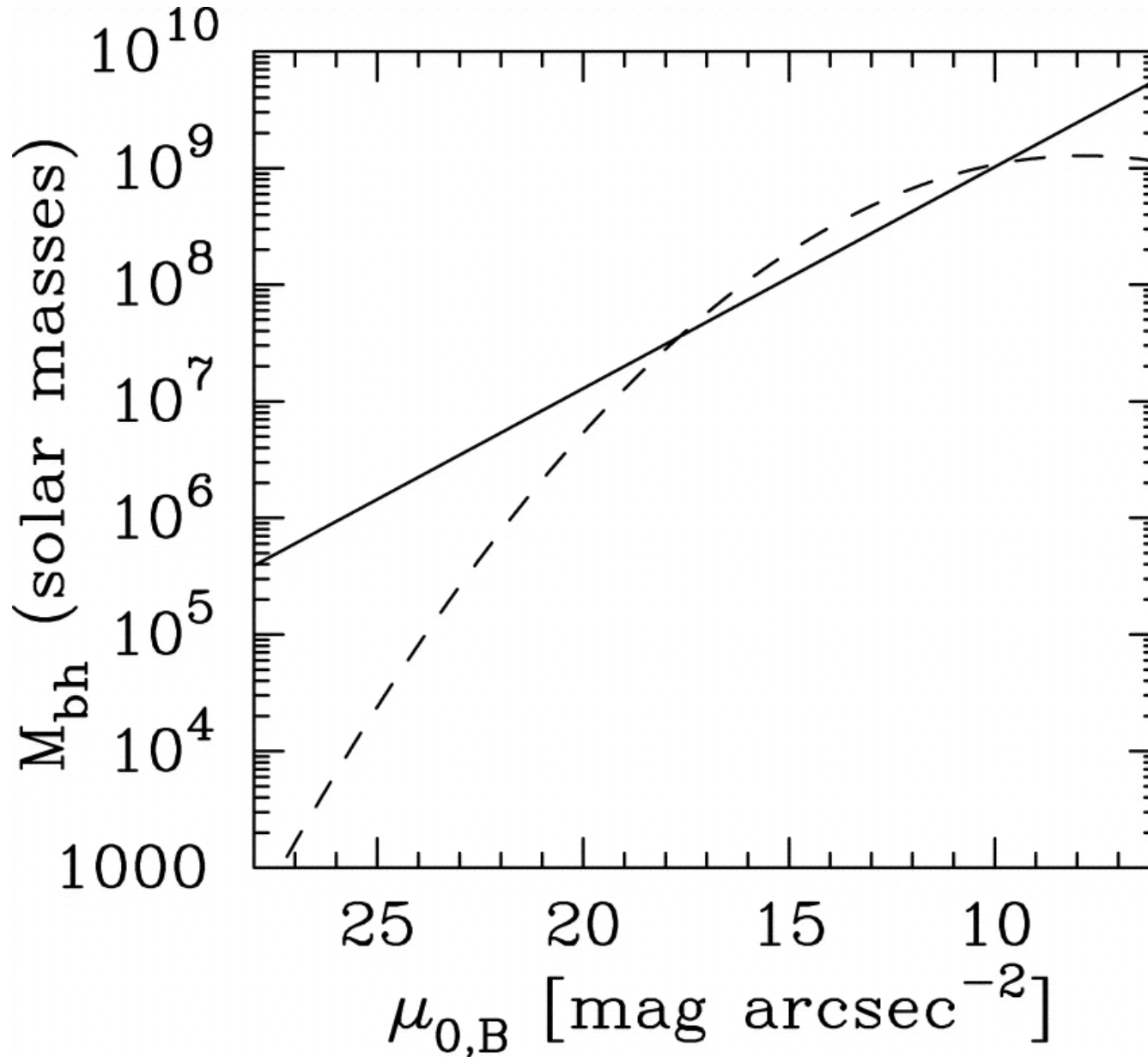
Fig. 4. from A LogQuadratic Relation for Predicting Supermassive Black Hole Masses from the Host Bulge Sérsic Index Graham & Driver 2007 ApJ 655 77 doi:10.1086/509758 https://dx.doi.org/10.1086/509758 © 2007. The American Astronomical Society. All rights reserved. Printed in U.S.A.
